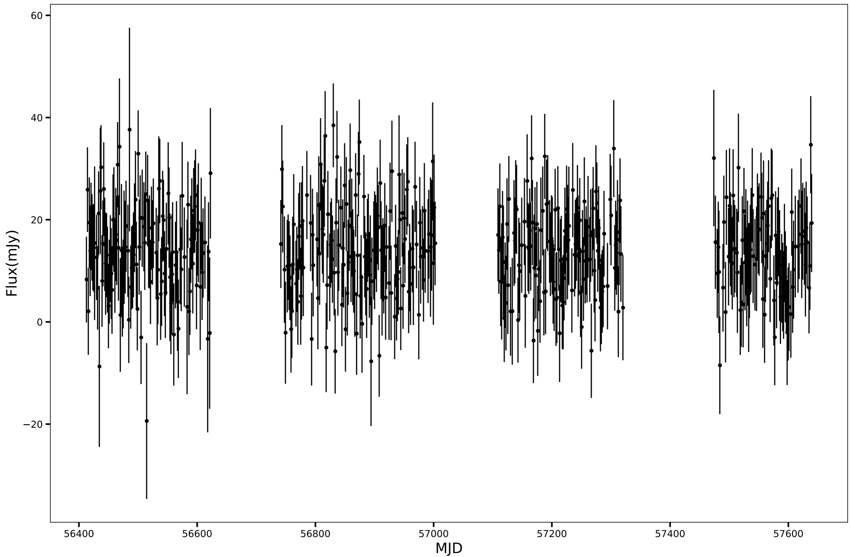
SPT-SJ002513-6028.5, RA=6.3064d, DEC=-60.4755d, mean_flux=13.70 (mJy)
