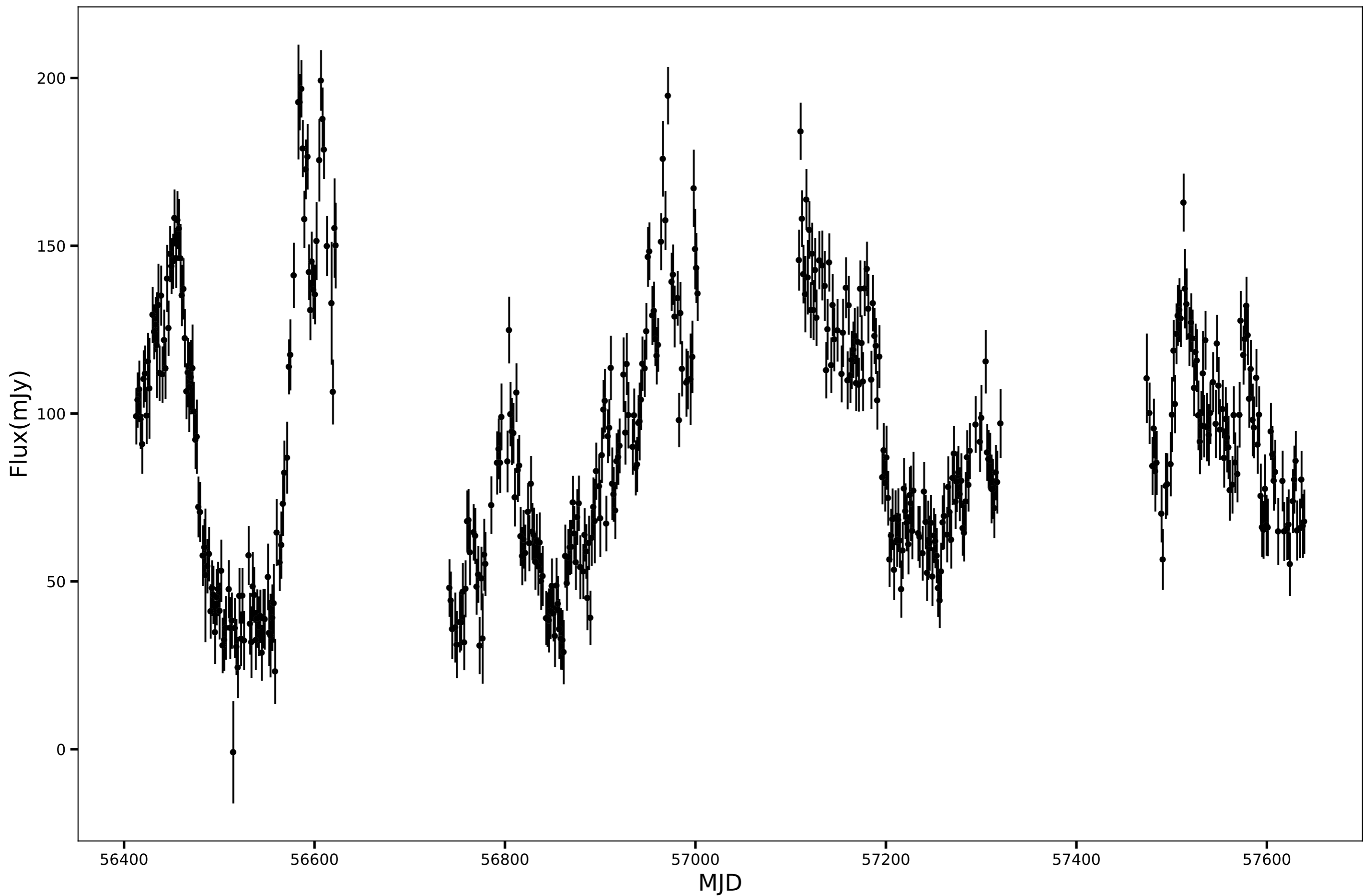
SPT-SJ002341-5930.5, RA=5.9250d, DEC=-59.5093d, mean_flux=90.80 (mJy)
