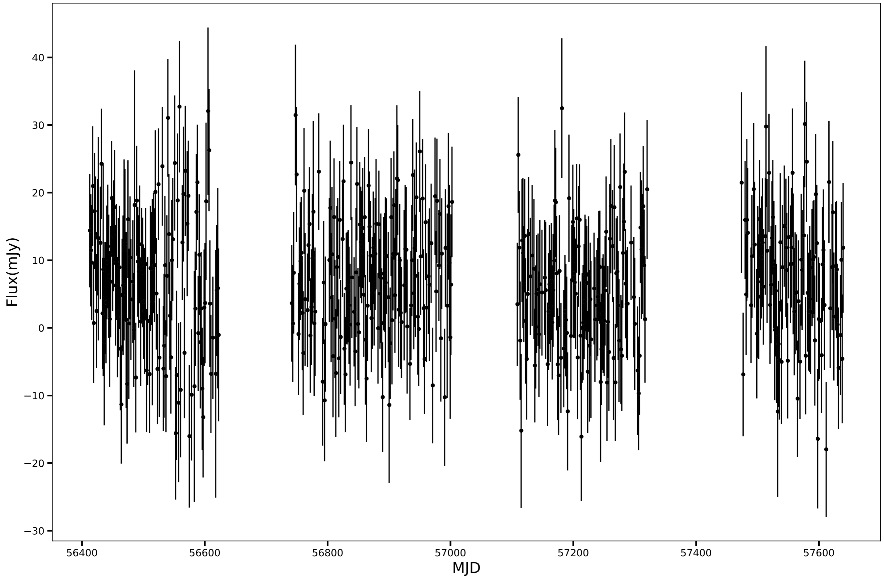
SPT-SJ002320-6046.3, RA=5.8361d, DEC=-60.7726d, mean_flux=6.61 (mJy)
