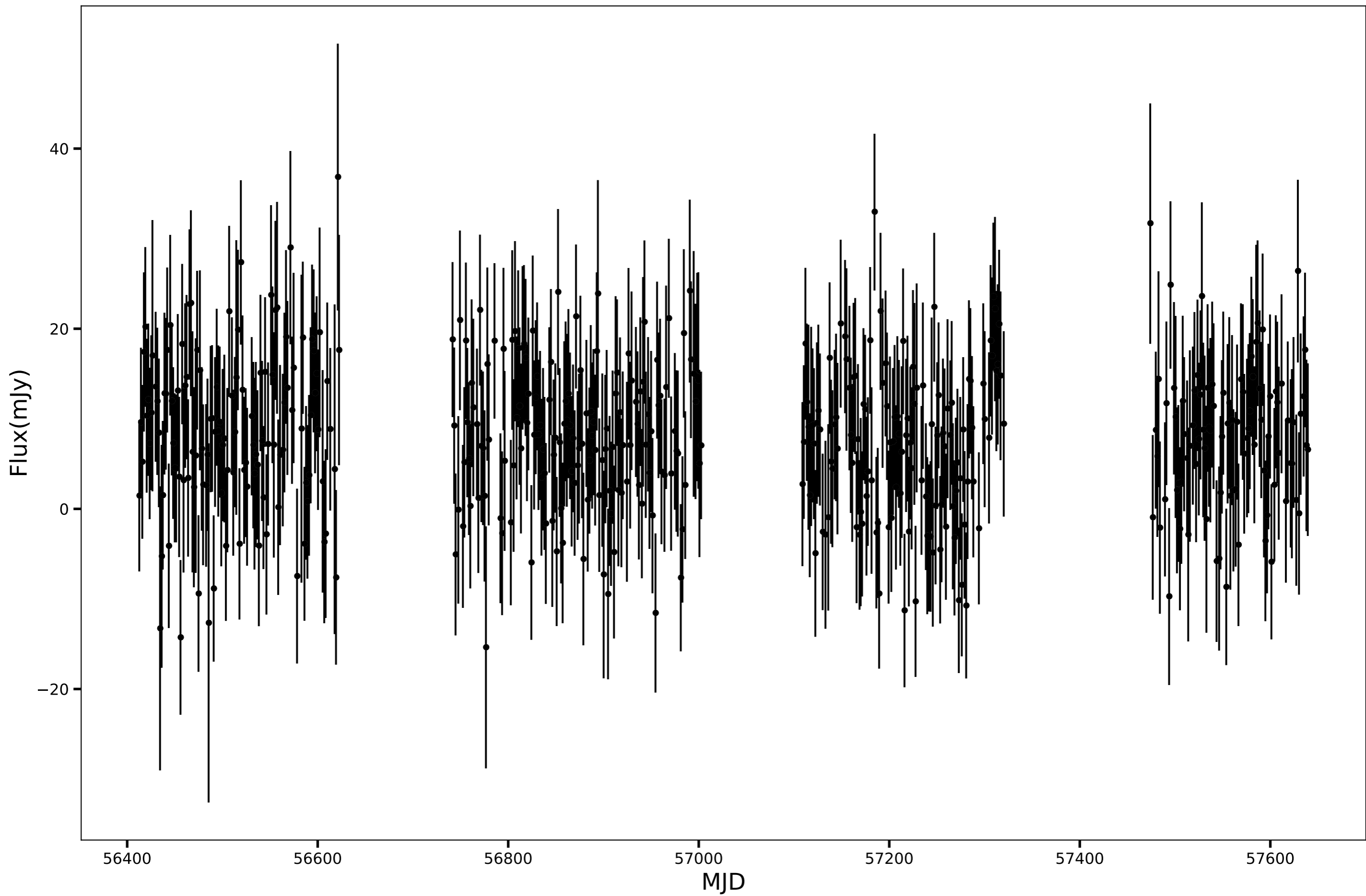
SPT-SJ002307-6507.0, RA=5.7803d, DEC=-65.1172d, mean_flux=7.95 (mJy)
