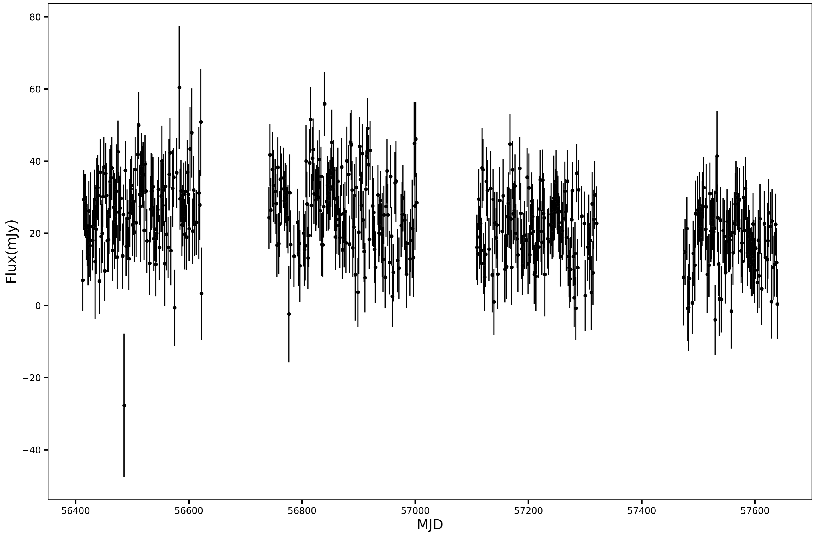
SPT-SJ002233-5153.2, RA=5.6387d, DEC=-51.8871d, mean_flux=23.39 (mJy)
