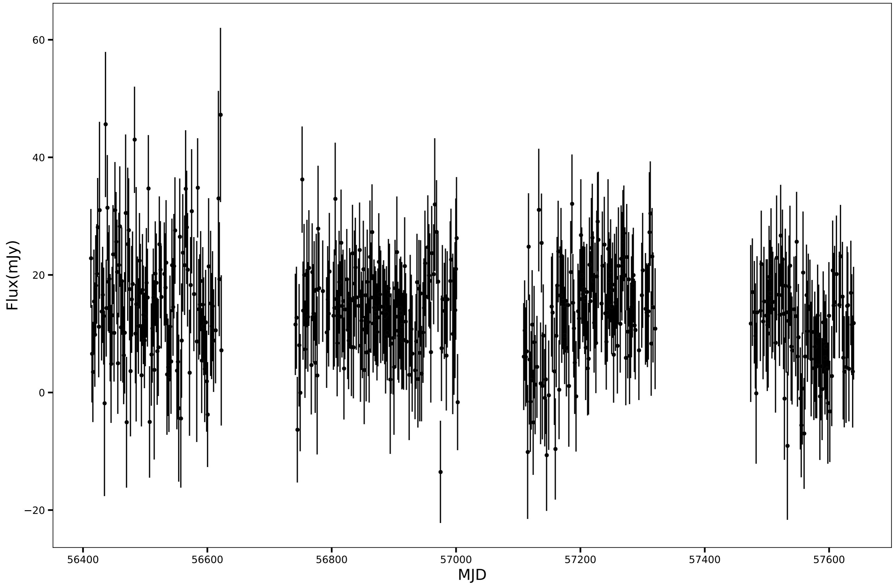
SPT-SJ001956-6253.1, RA=4.9851d, DEC=-62.8855d, mean_flux=13.75 (mJy)
