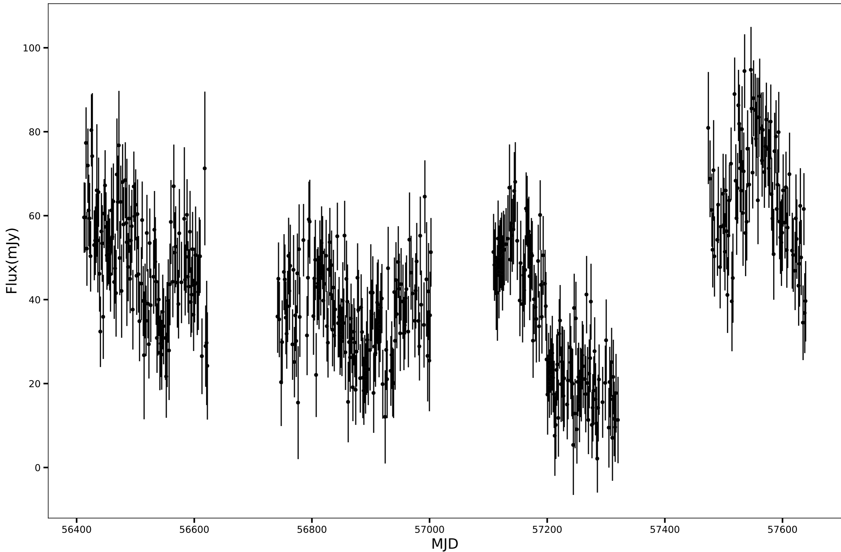
SPT-SJ001926-5641.7, RA=4.8610d, DEC=-56.6961d, mean_flux=44.14 (mJy)
