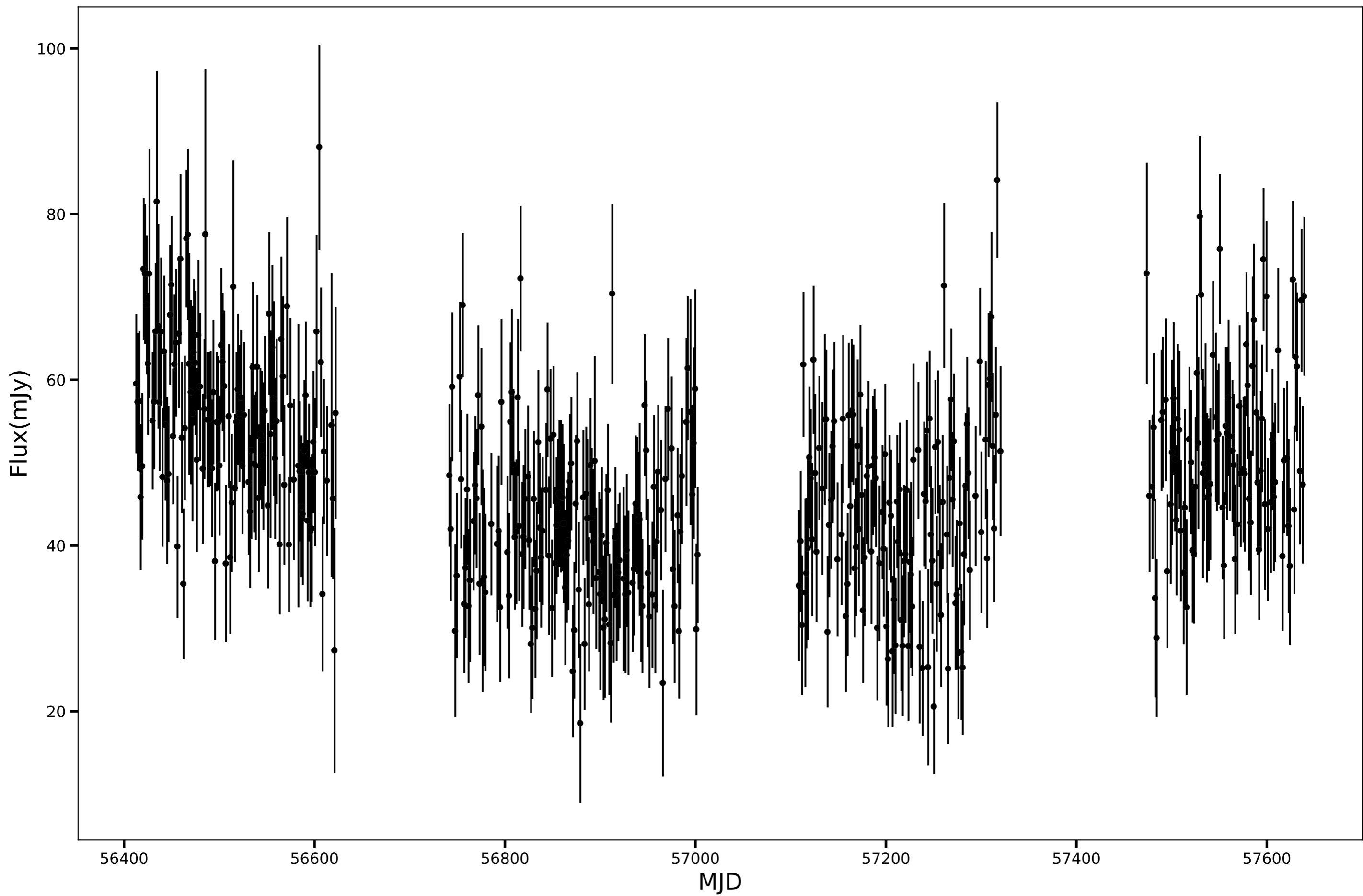
SPT-SJ001848-5115.0, RA=4.7015d, DEC=-51.2506d, mean_flux=47.84 (mJy)
