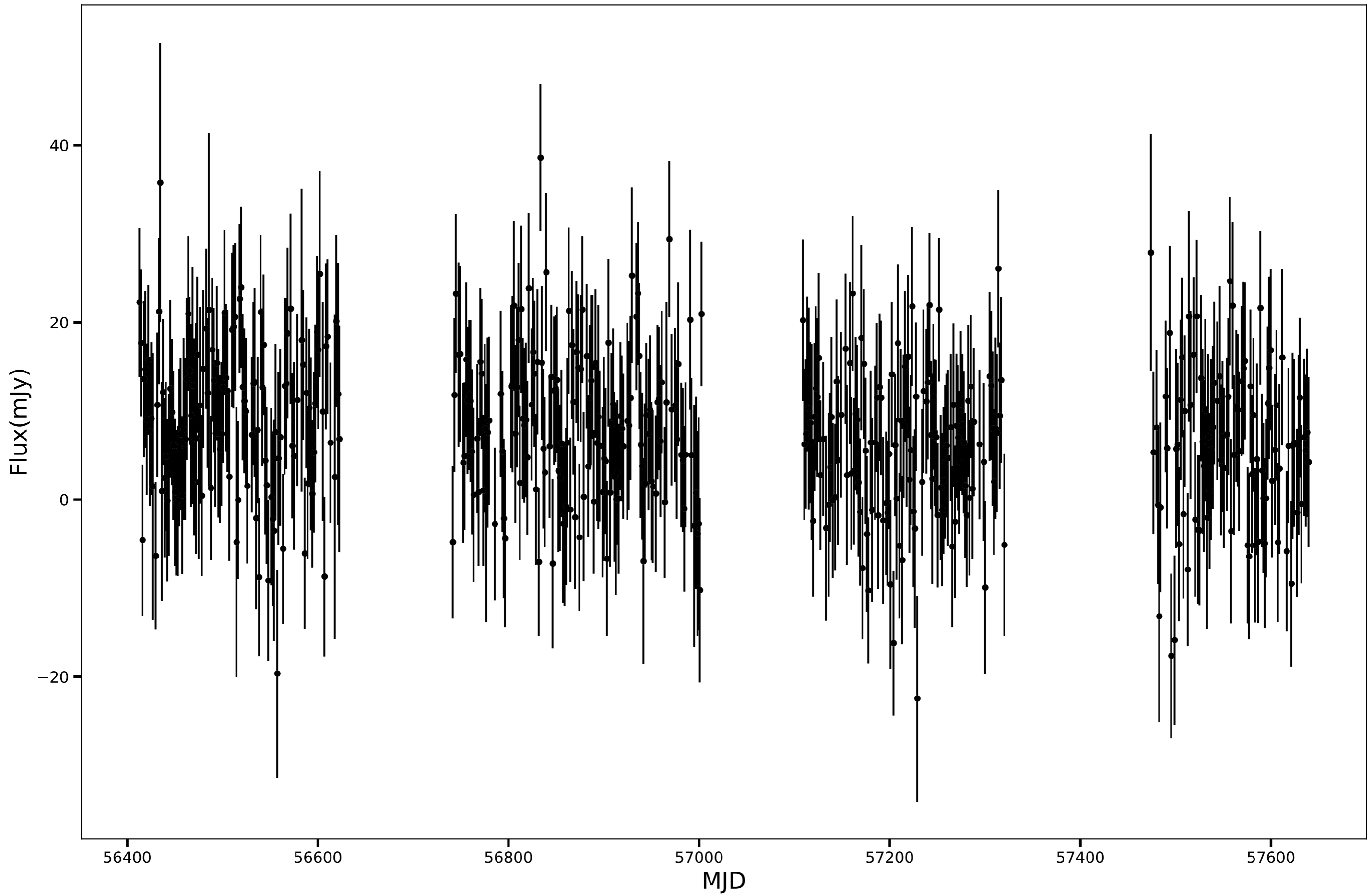
SPT-SJ001601-6310.1, RA=4.0061d, DEC=-63.1687d, mean_flux=7.45 (mJy)
