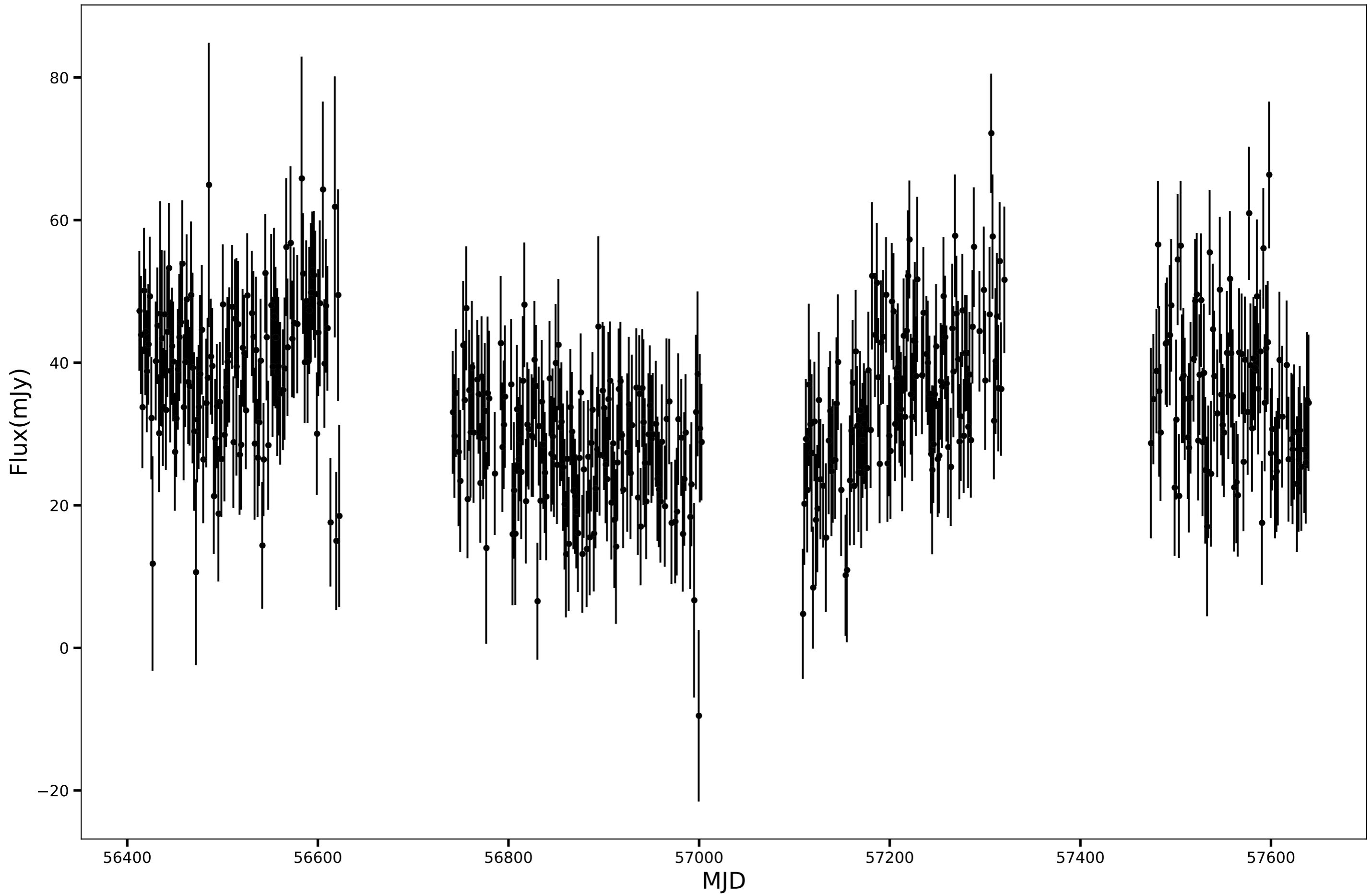
SPT-SJ001426-5638.4, RA=3.6122d, DEC=-56.6404d, mean_flux=34.42 (mJy)
