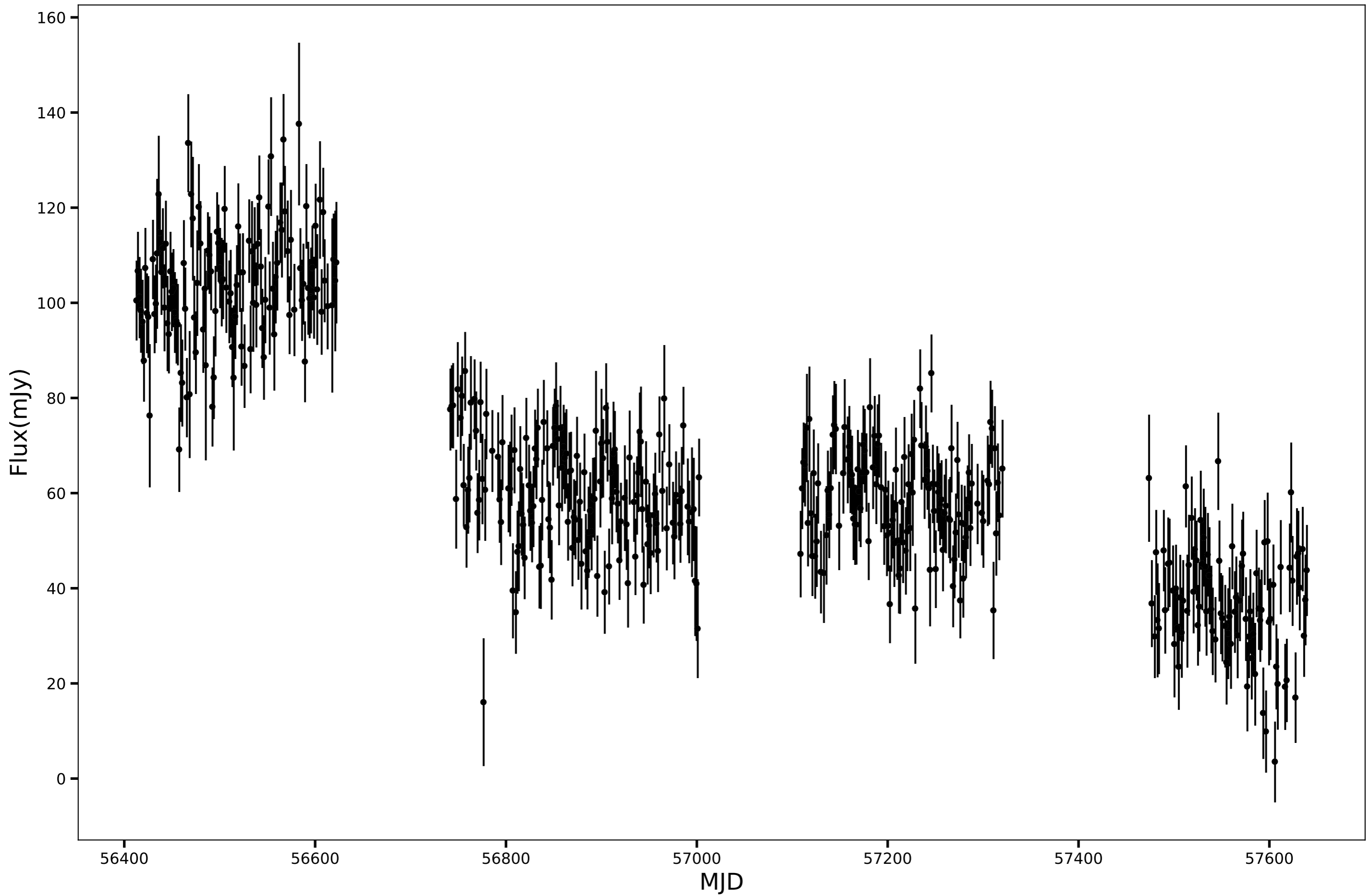
SPT-SJ001324-5005.2, RA=3.3516d, DEC=-50.0877d, mean_flux=66.54 (mJy)
