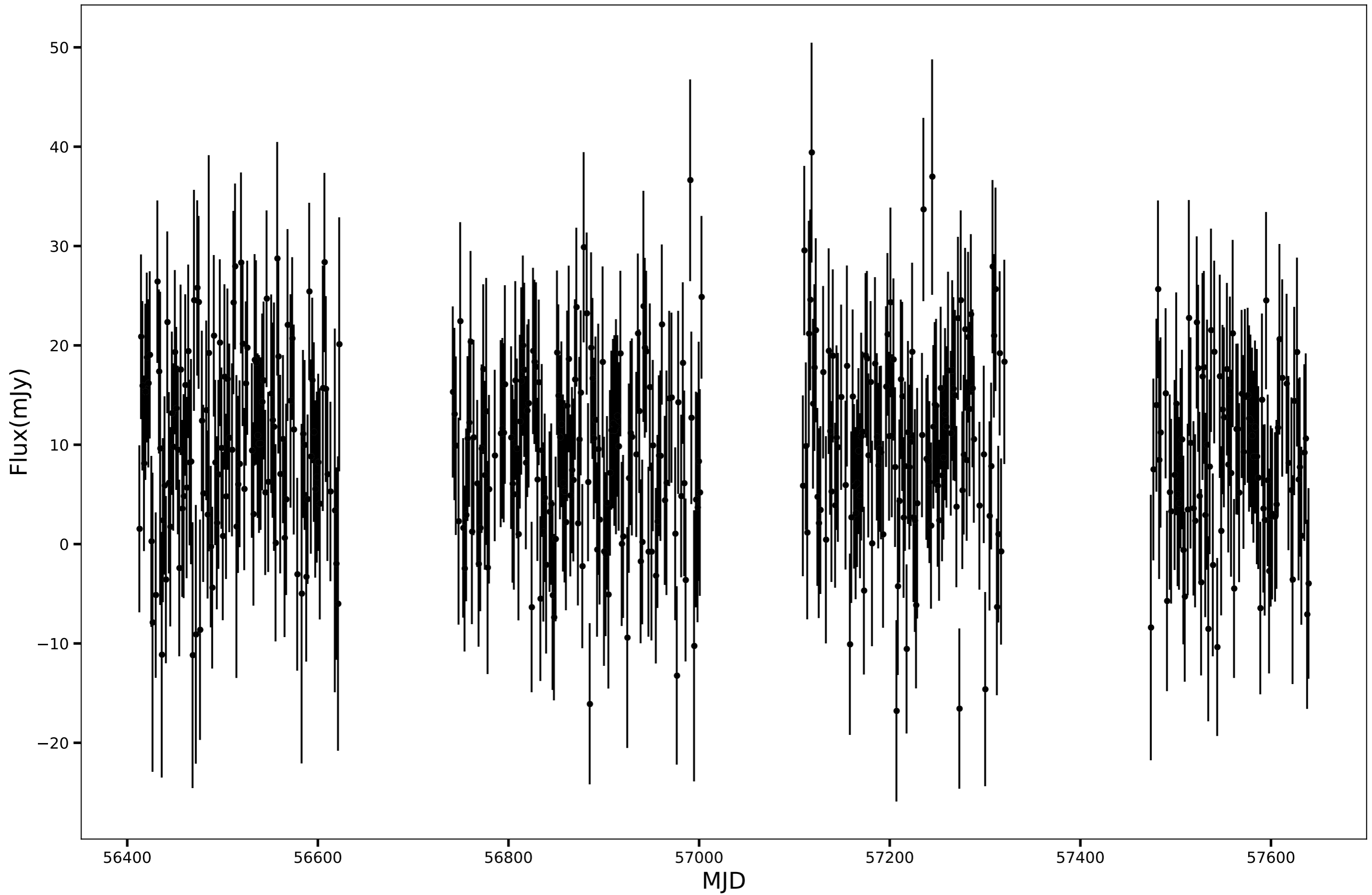
SPT-SJ001317-5610.6, RA=3.3240d, DEC=-56.1773d, mean_flux=9.50 (mJy)
