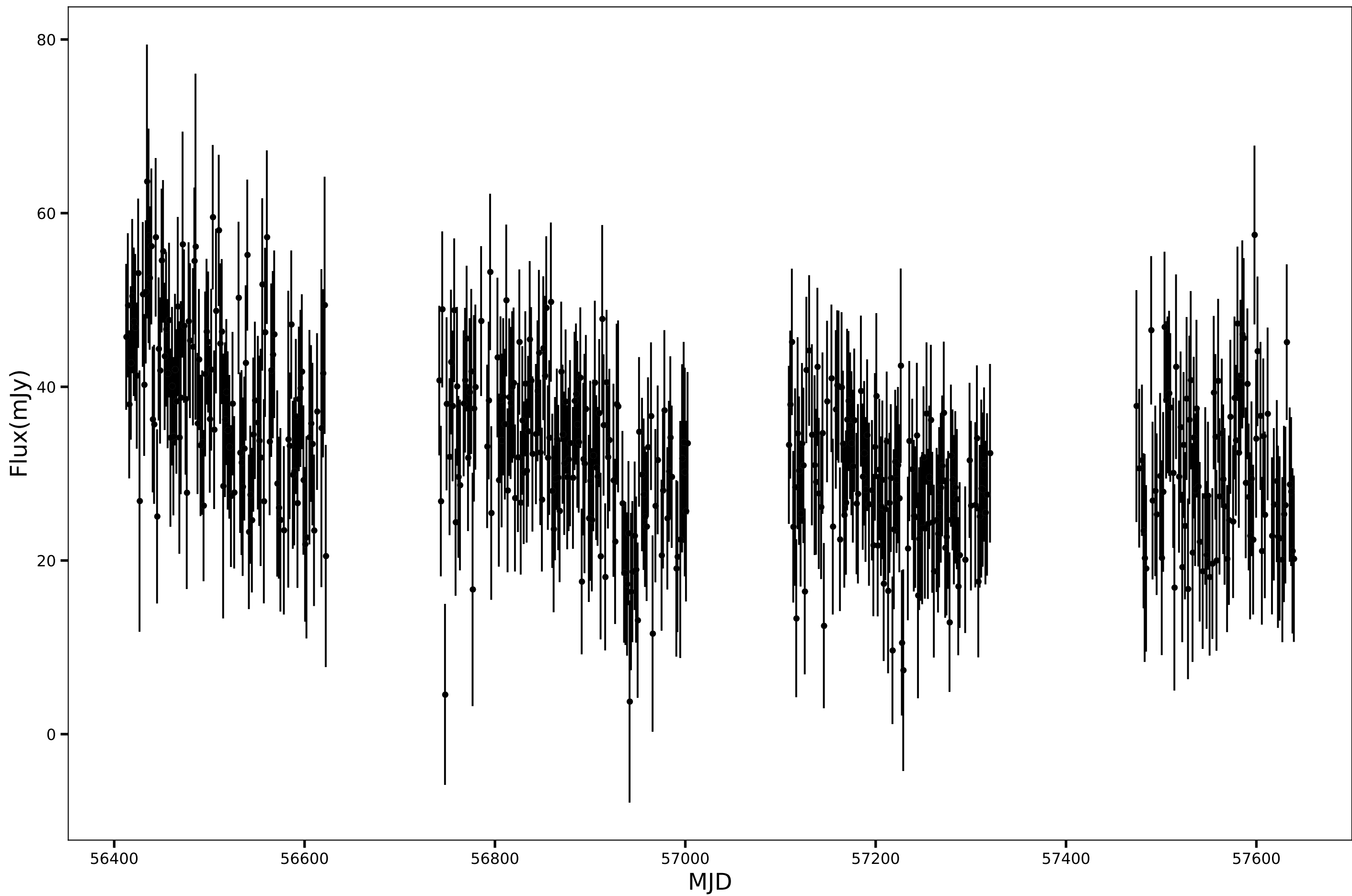
SPT-SJ000936-6357.5, RA=2.4031d, DEC=-63.9591d, mean_flux=32.91 (mJy)
