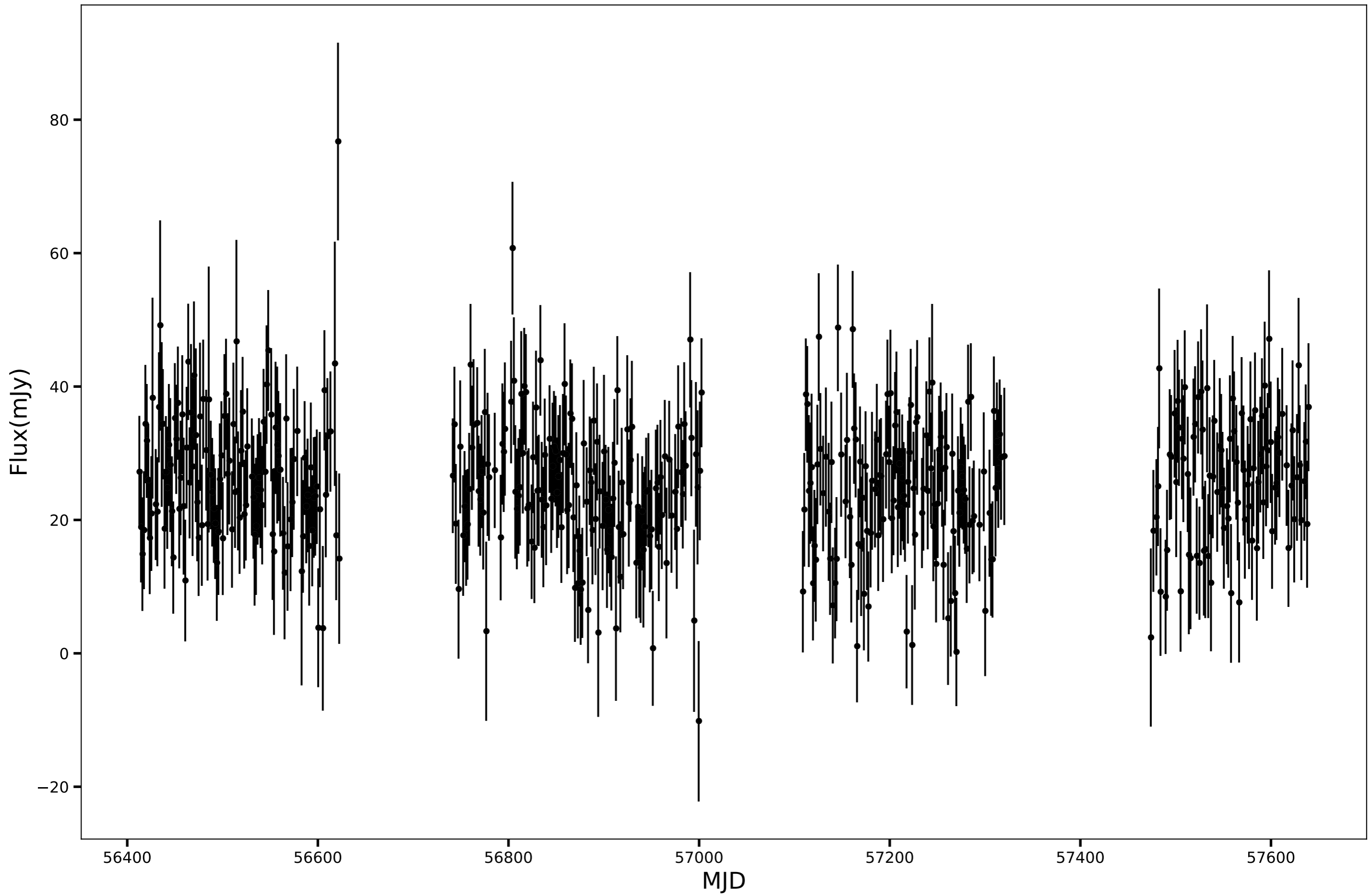
SPT-SJ000922-5130.2, RA=2.3420d, DEC=-51.5046d, mean_flux=25.33 (mJy)
