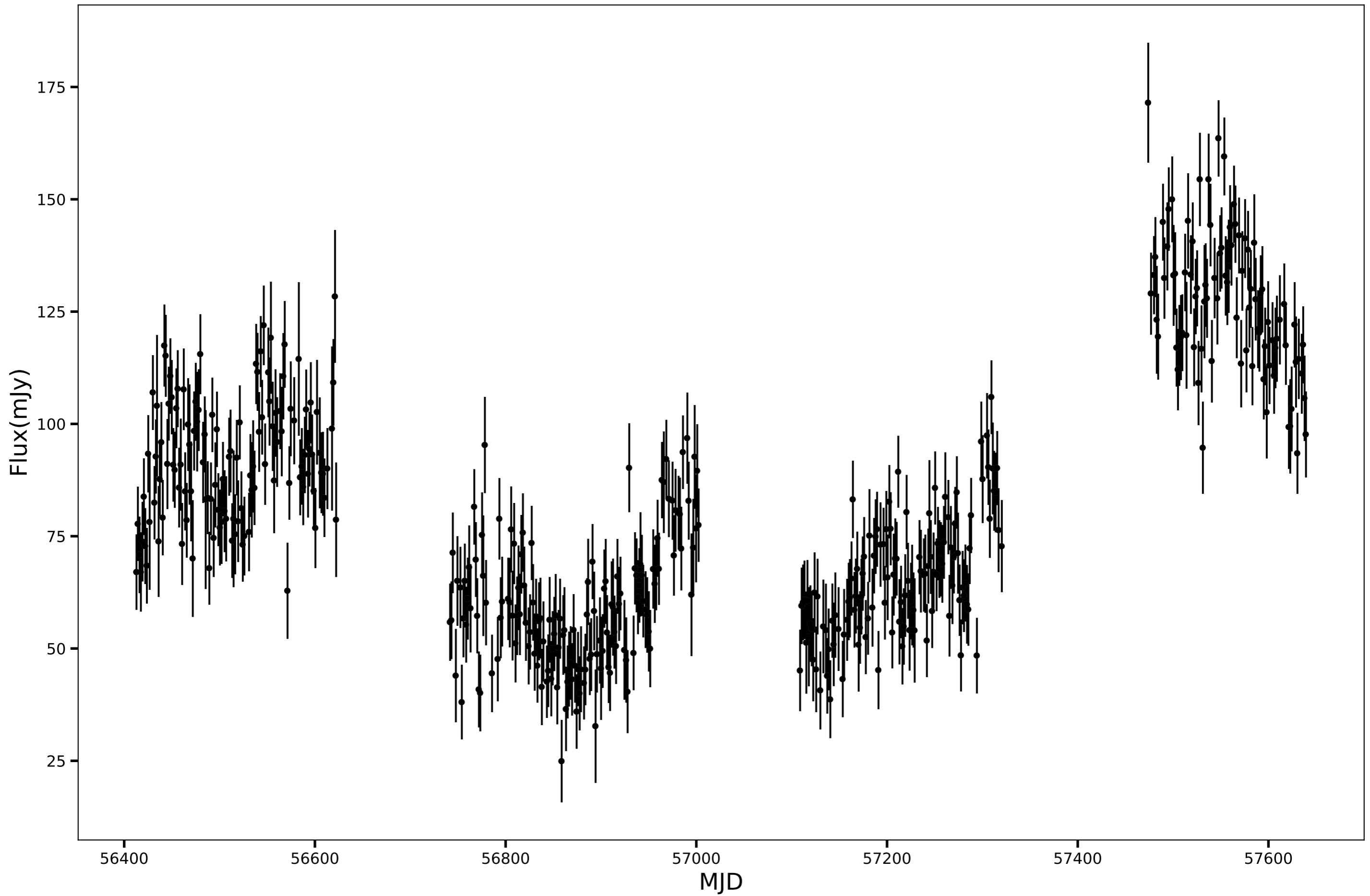
SPT-SJ000800-5243.6, RA=2.0027d, DEC=-52.7277d, mean_flux=82.17 (mJy)
