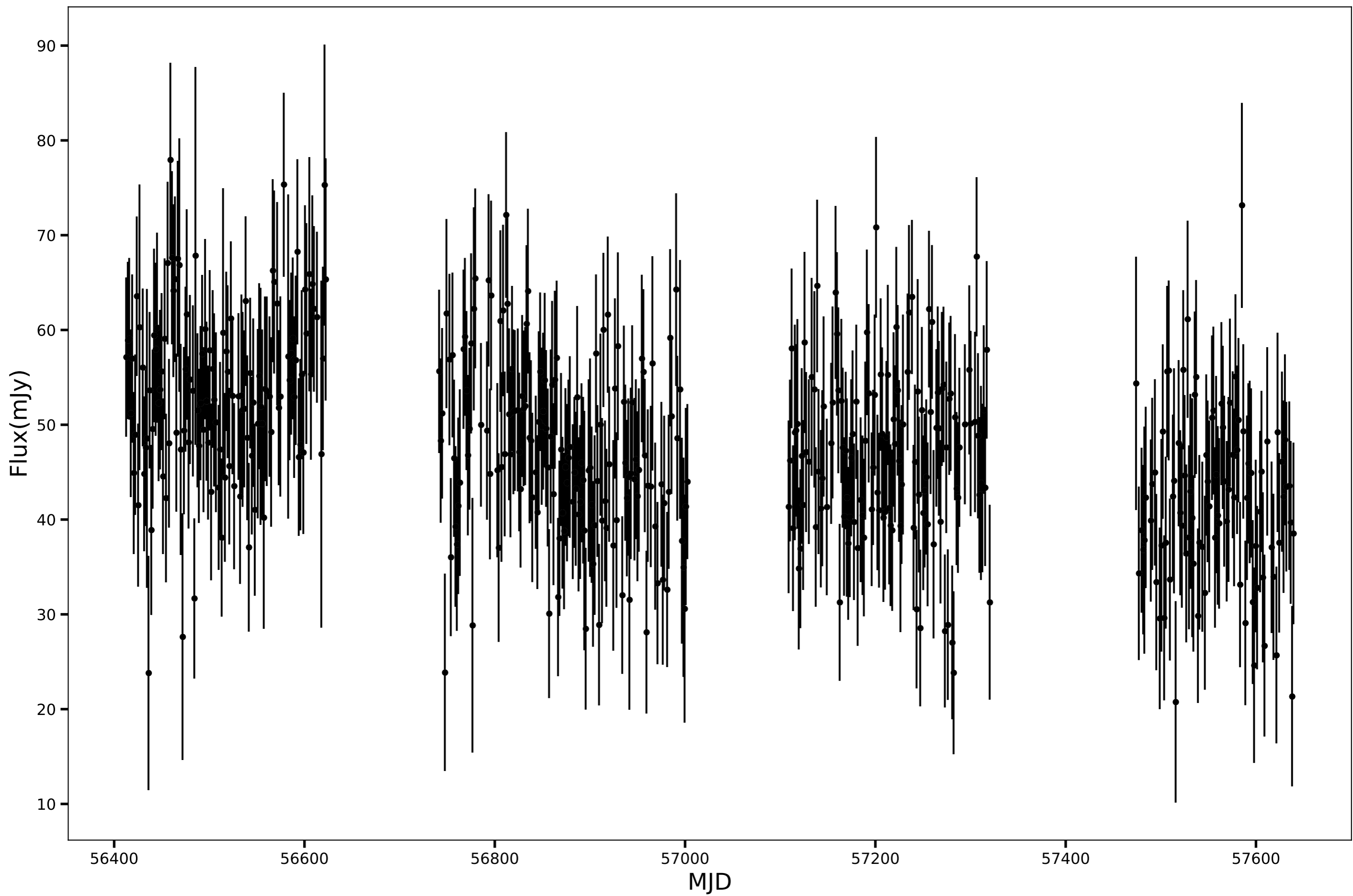
SPT-SJ000719-6113.2, RA=1.8315d, DEC=-61.2210d, mean_flux=47.78 (mJy)
