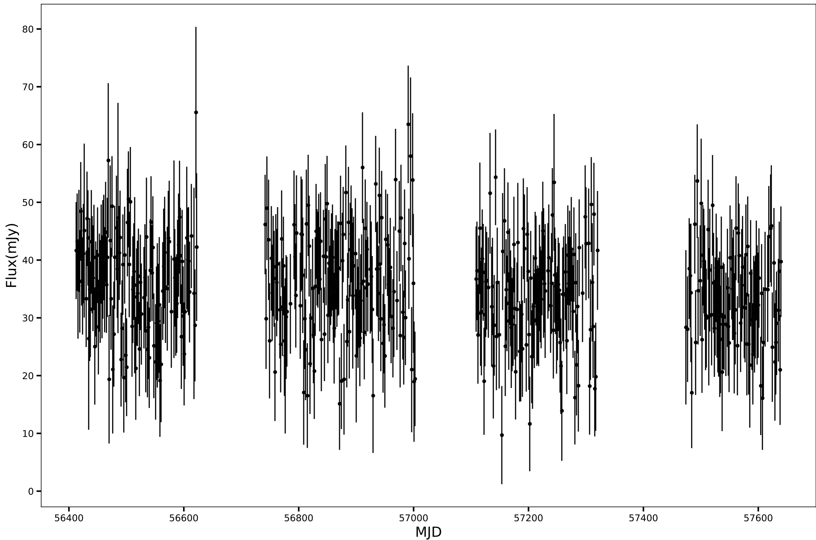
SPT-SJ000558-5628.5, RA=1.4924d, DEC=-56.4755d, mean_flux=34.95 (mJy)
