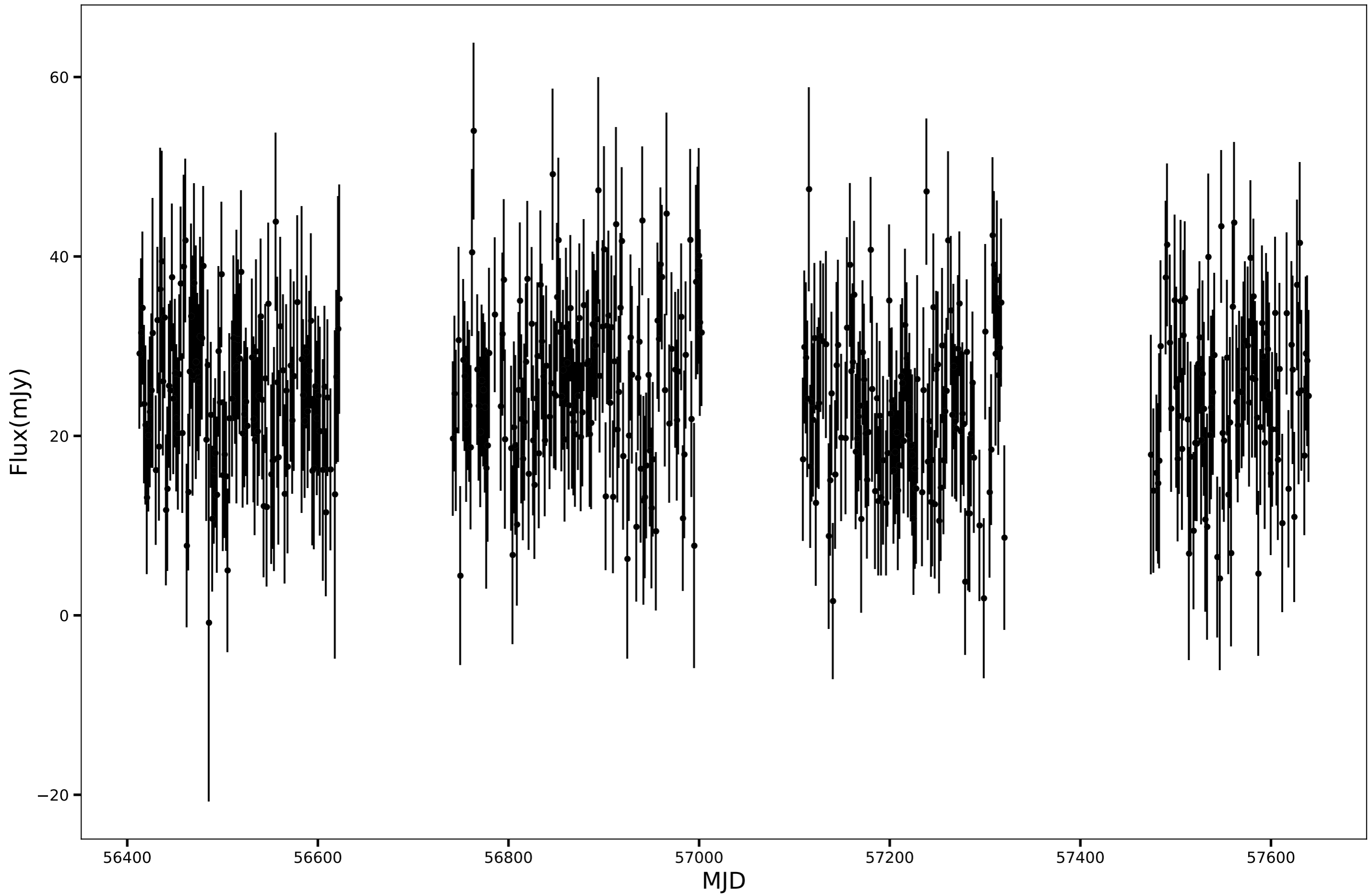
SPT-SJ000413-5255.0, RA=1.0576d, DEC=-52.9170d, mean_flux=24.51 (mJy)
