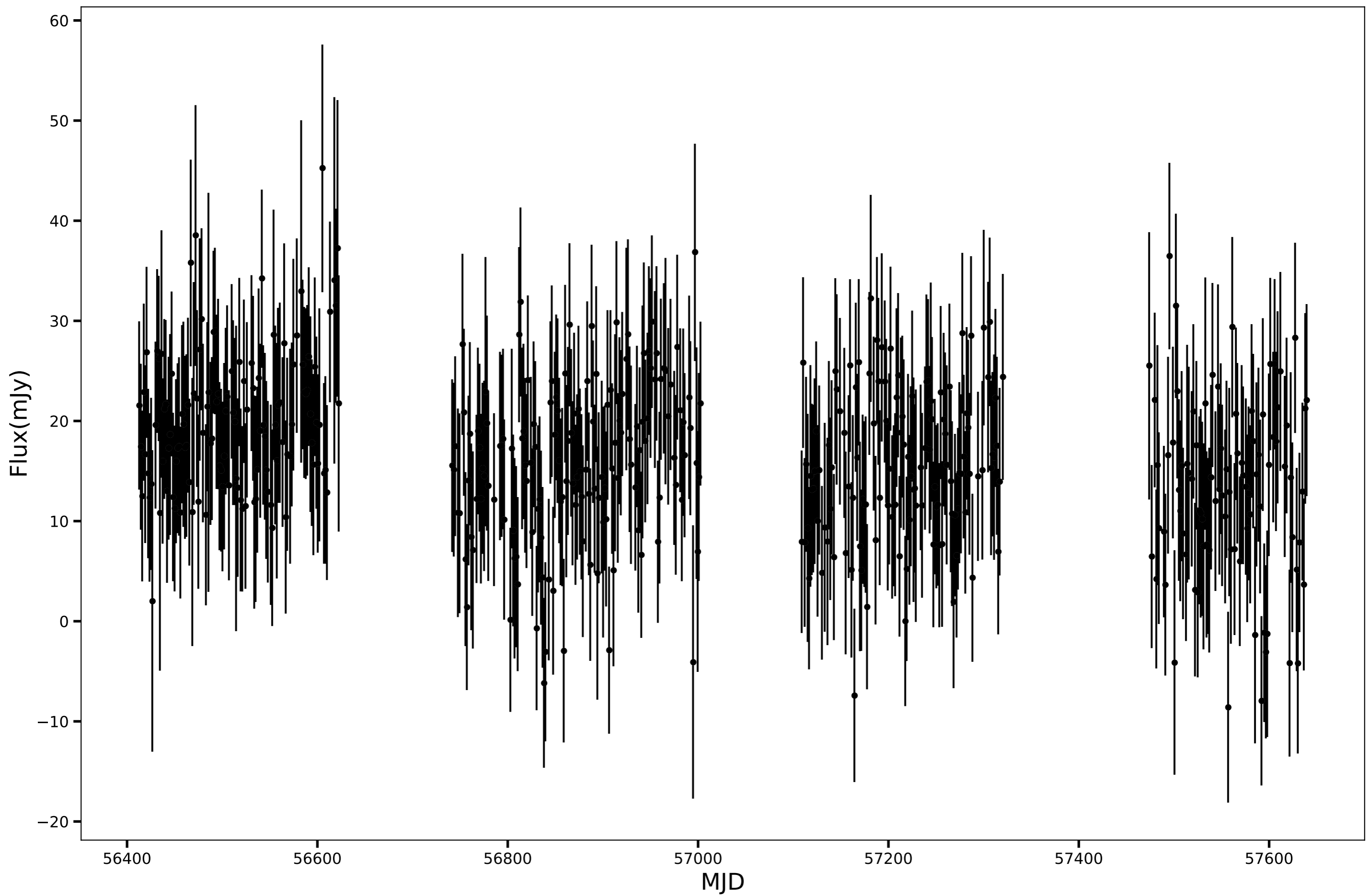
SPT-SJ000312-5905.7, RA=0.8038d, DEC=-59.0958d, mean_flux=16.27 (mJy)
