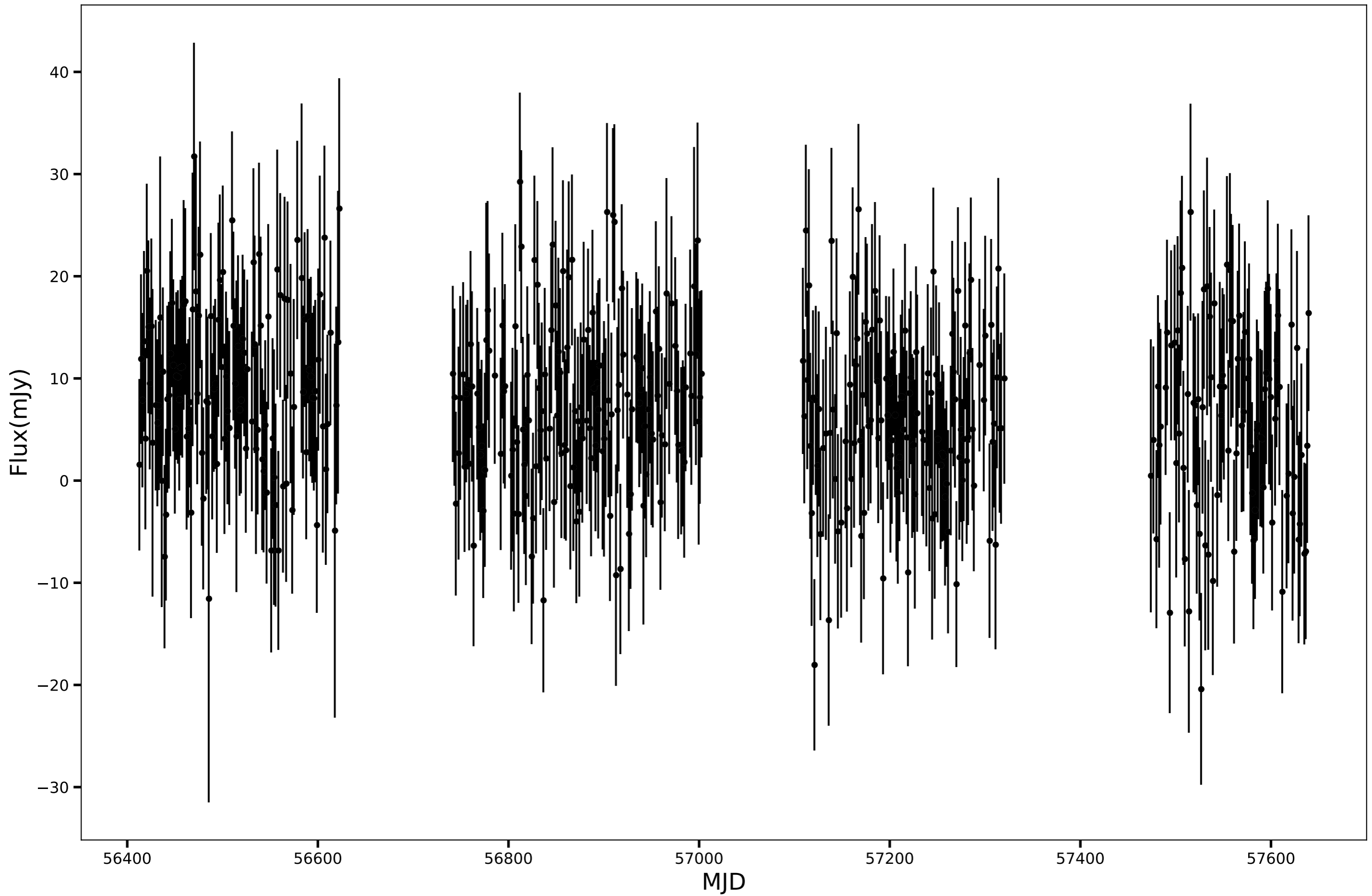
SPT-SJ000254-5621.0, RA=0.7251d, DEC=-56.3513d, mean_flux=7.25 (mJy)
