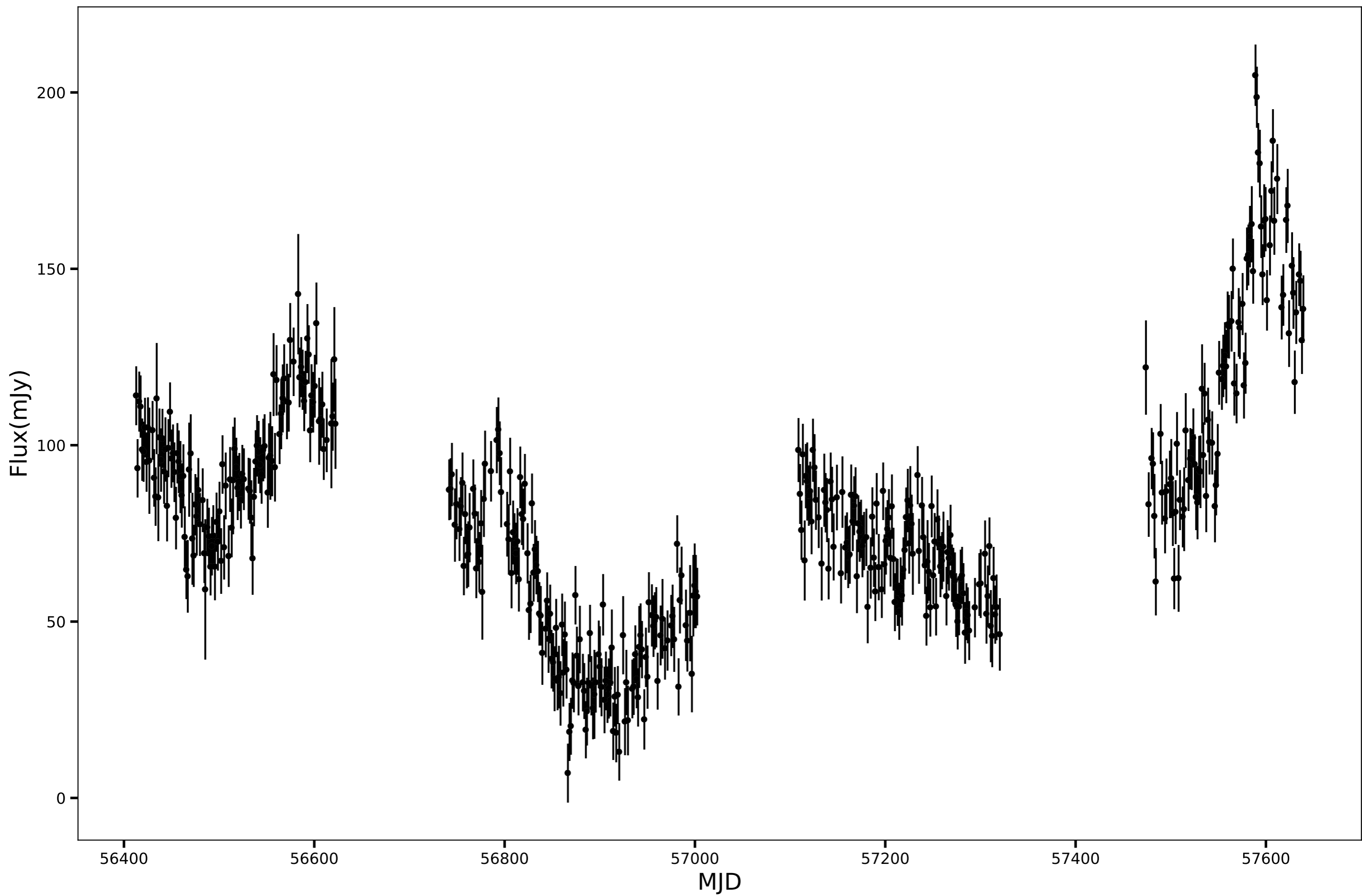
SPT-SJ000252-5948.0, RA=0.7198d, DEC=-59.8015d, mean_flux=81.10 (mJy)
