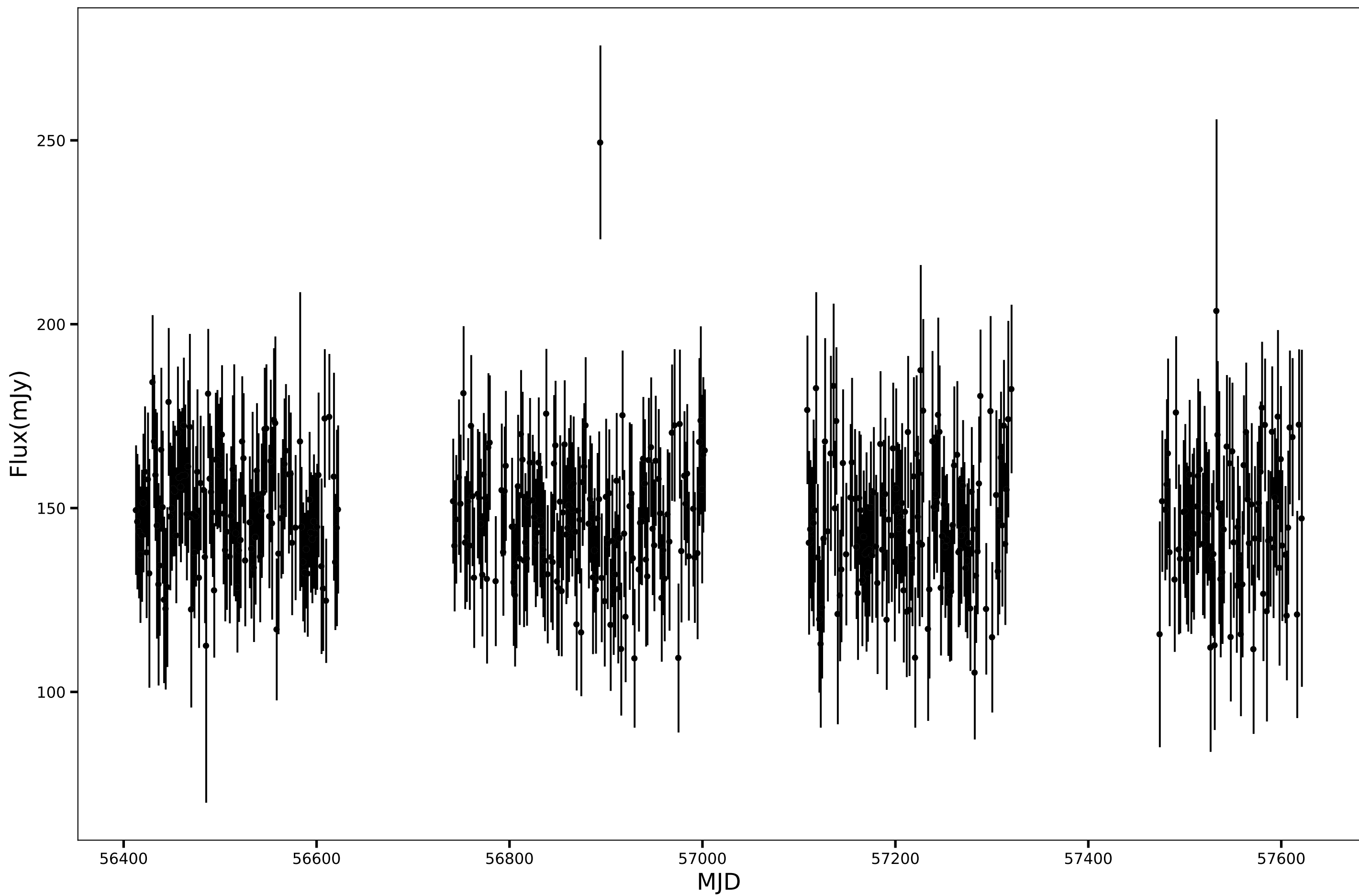
SPT-SJ235920-6057.0, RA=359.8371d, DEC=-60.9500d, mean_flux=147.53 (mJy), 90GHz
