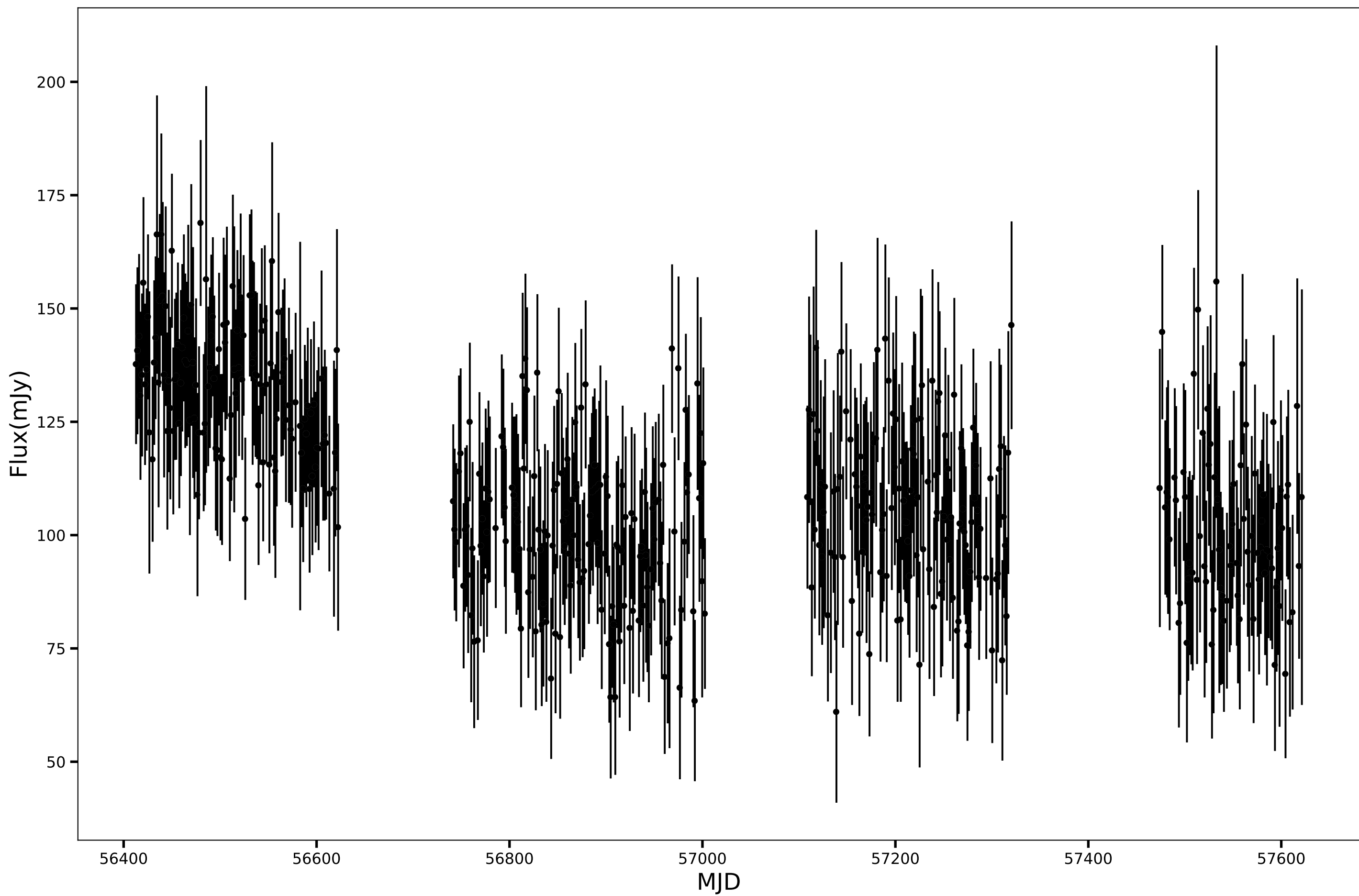
SPT-SJ235903-6055.1, RA=359.7654d, DEC=-60.9192d, mean_flux=110.45 (mJy), 90GHz
