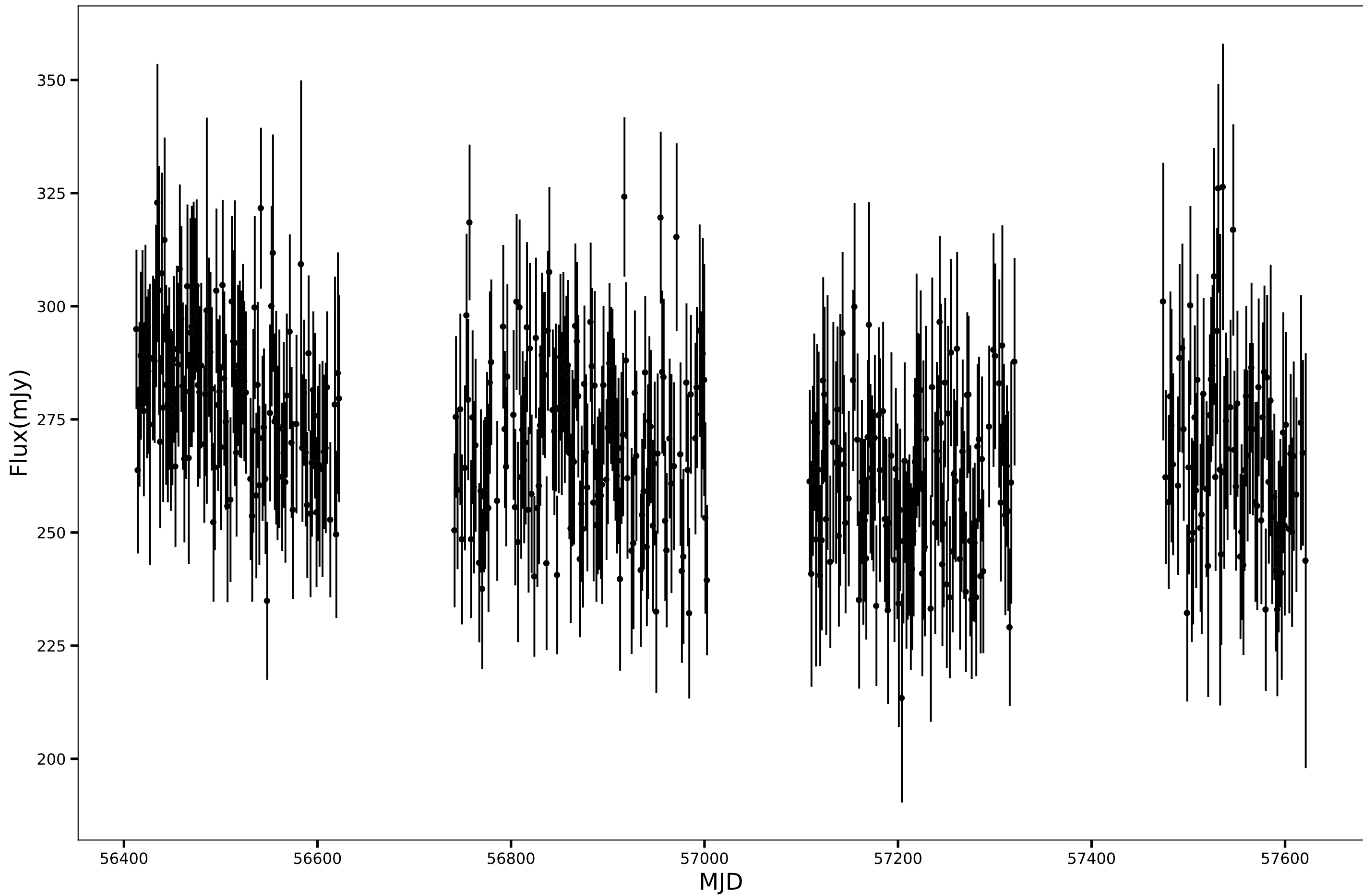
SPT-SJ235844-6053.0, RA=359.6871d, DEC=-60.8845d, mean_flux=269.92 (mJy), 90GHz
