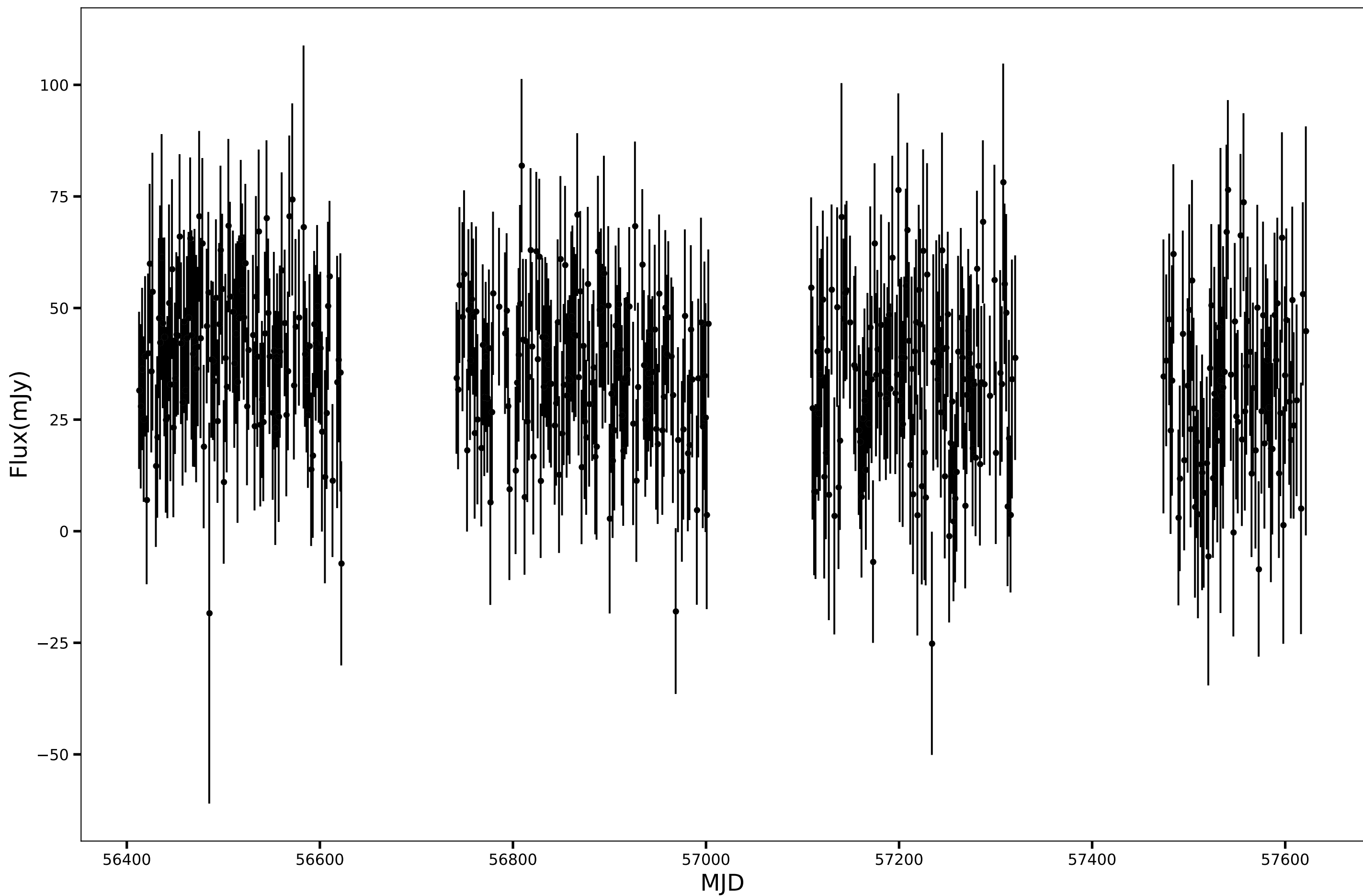
SPT-SJ235322-5857.3, RA=358.3446d, DEC=-58.9559d, mean_flux=35.56 (mJy), 90GHz
