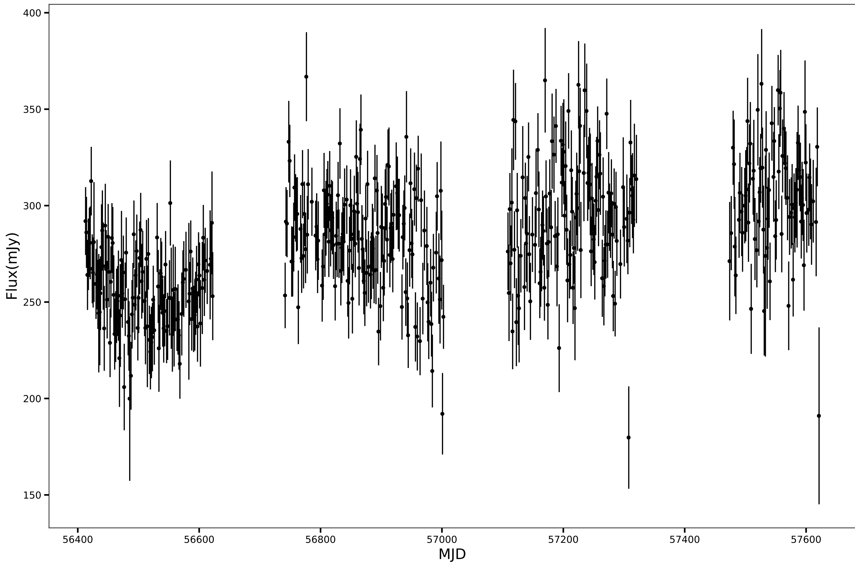
SPT-SJ234925-4932.4, RA=357.3583d, DEC=-49.5408d, mean_flux=282.25 (mJy), 90GHz
