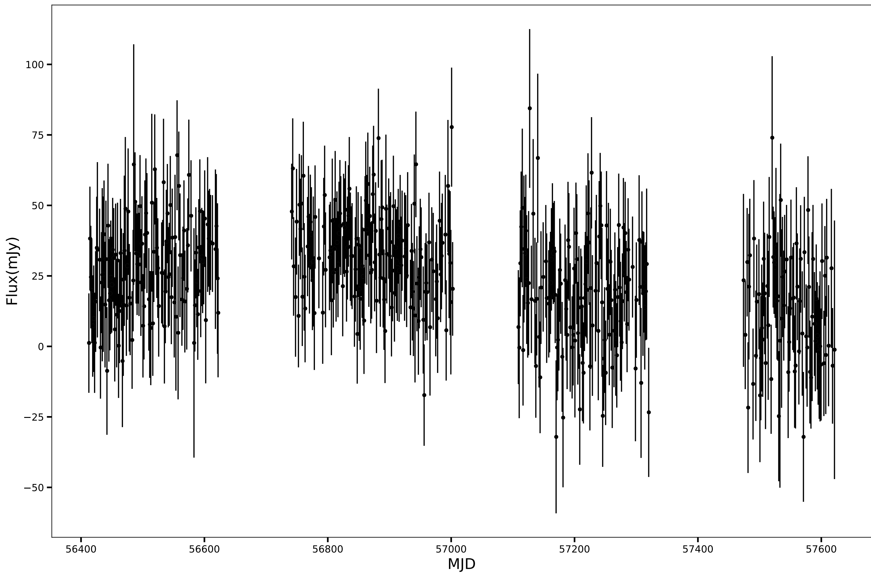
SPT-SJ234845-5847.0, RA=357.1886d, DEC=-58.7842d, mean_flux=24.01 (mJy), 90GHz
