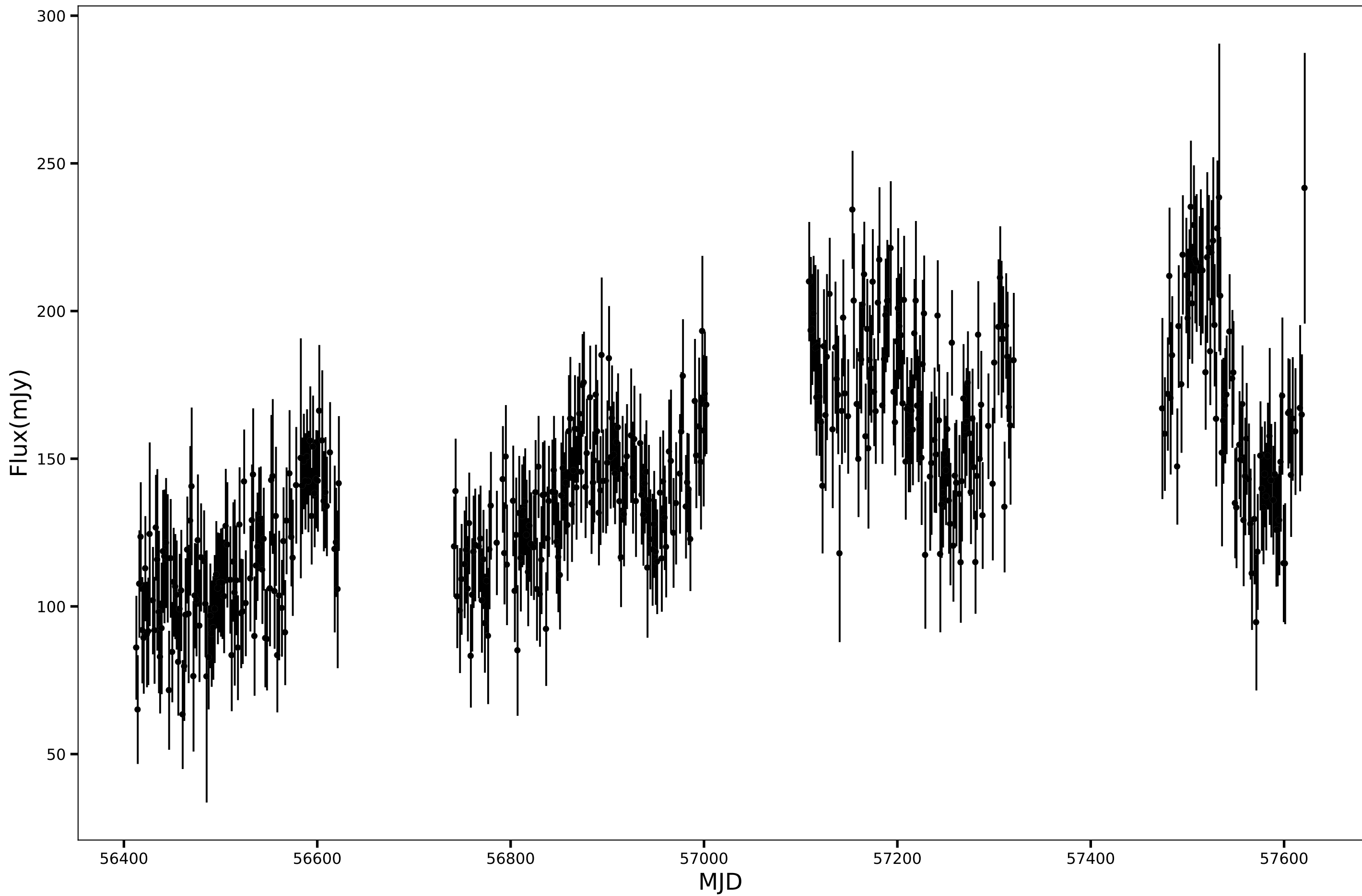
SPT-SJ234825-6049.2, RA=357.1046d, DEC=-60.8211d, mean_flux=144.86 (mJy), 90GHz
