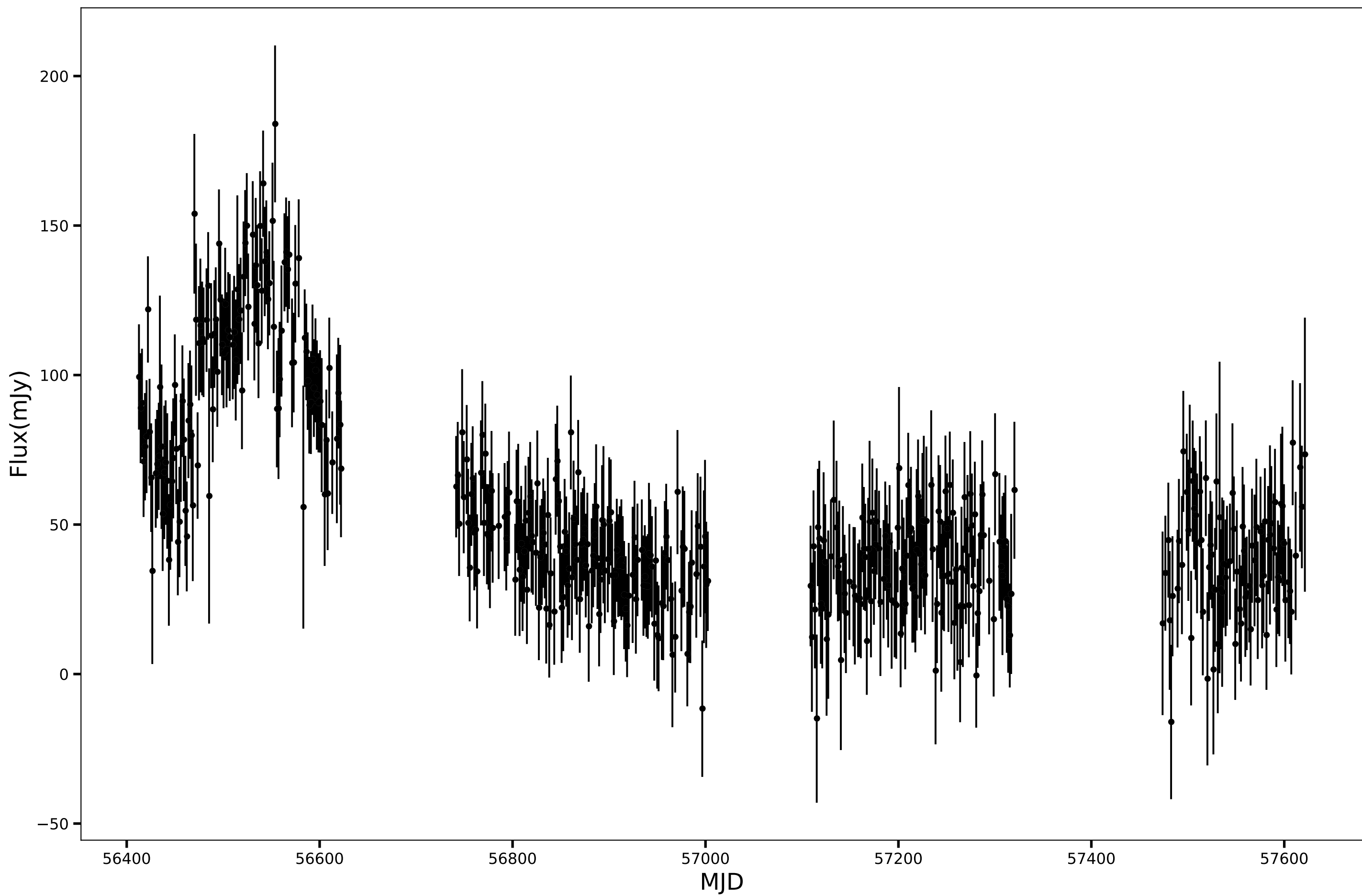
SPT-SJ234751-5915.5, RA=356.9662d, DEC=-59.2597d, mean_flux=54.62 (mJy), 90GHz
