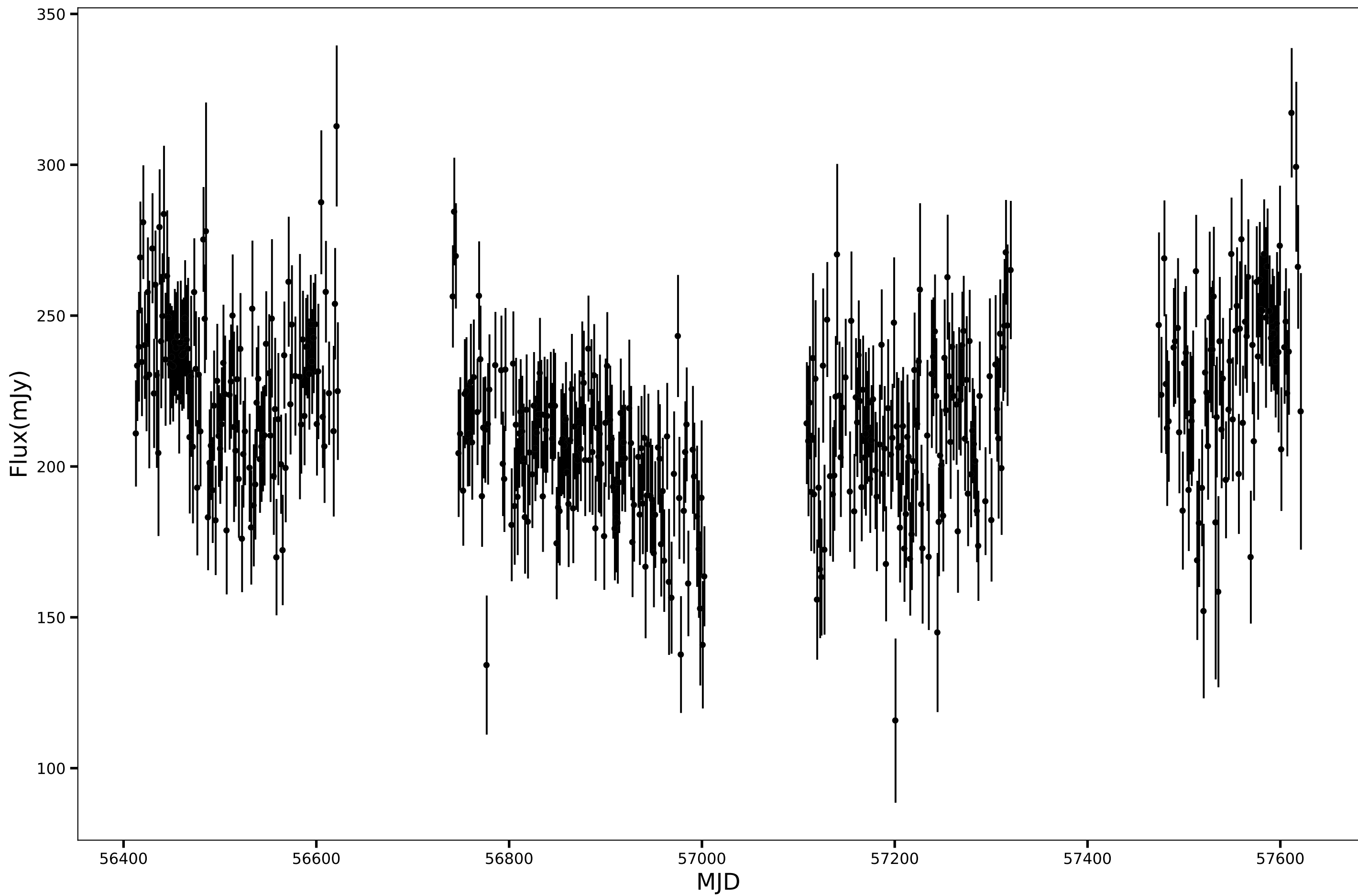
SPT-SJ234743-4946.4, RA=356.9326d, DEC=-49.7745d, mean_flux=216.85 (mJy), 90GHz
