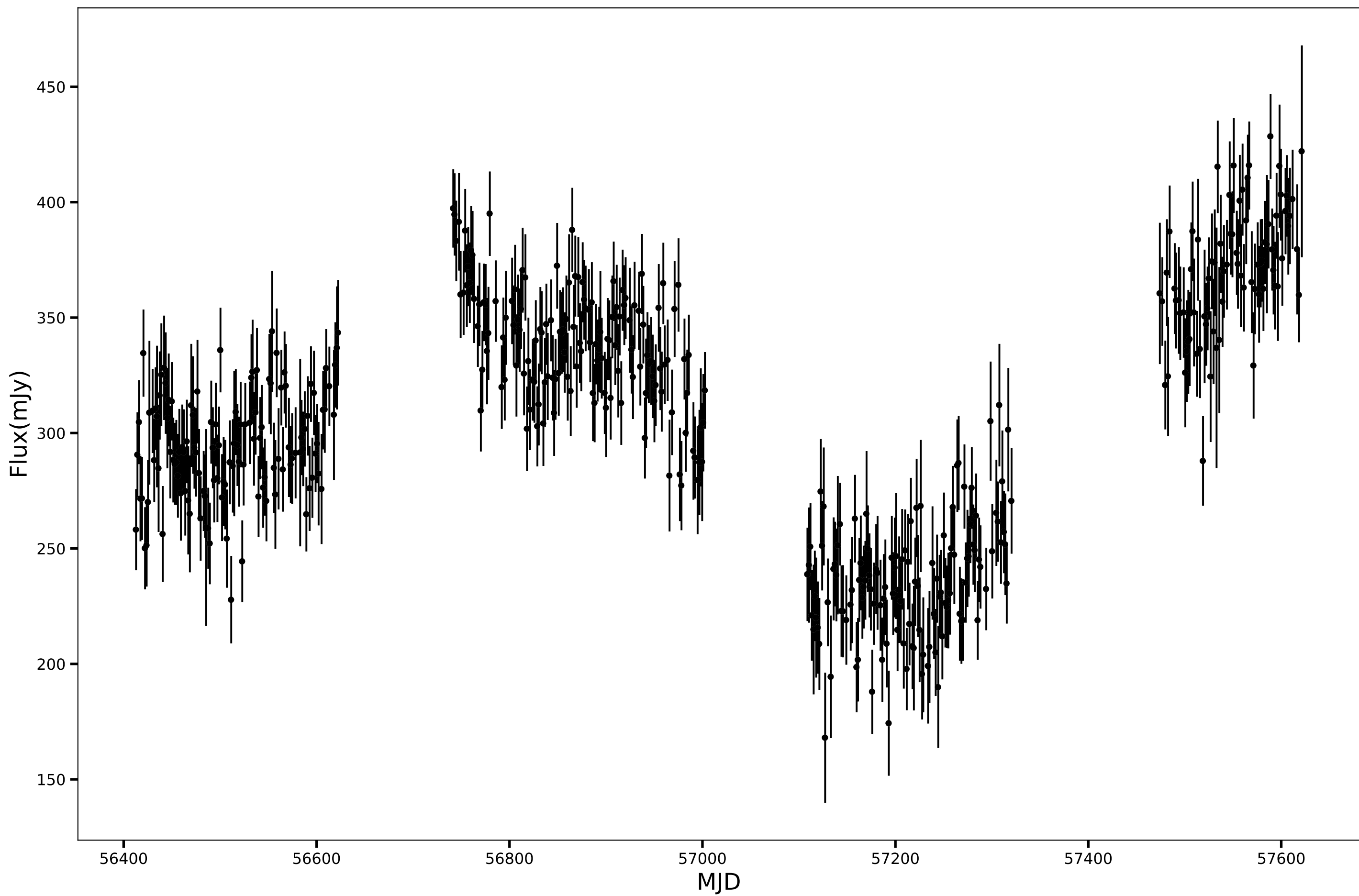
SPT-SJ234720-5110.6, RA=356.8338d, DEC=-51.1769d, mean_flux=305.92 (mJy), 90GHz
