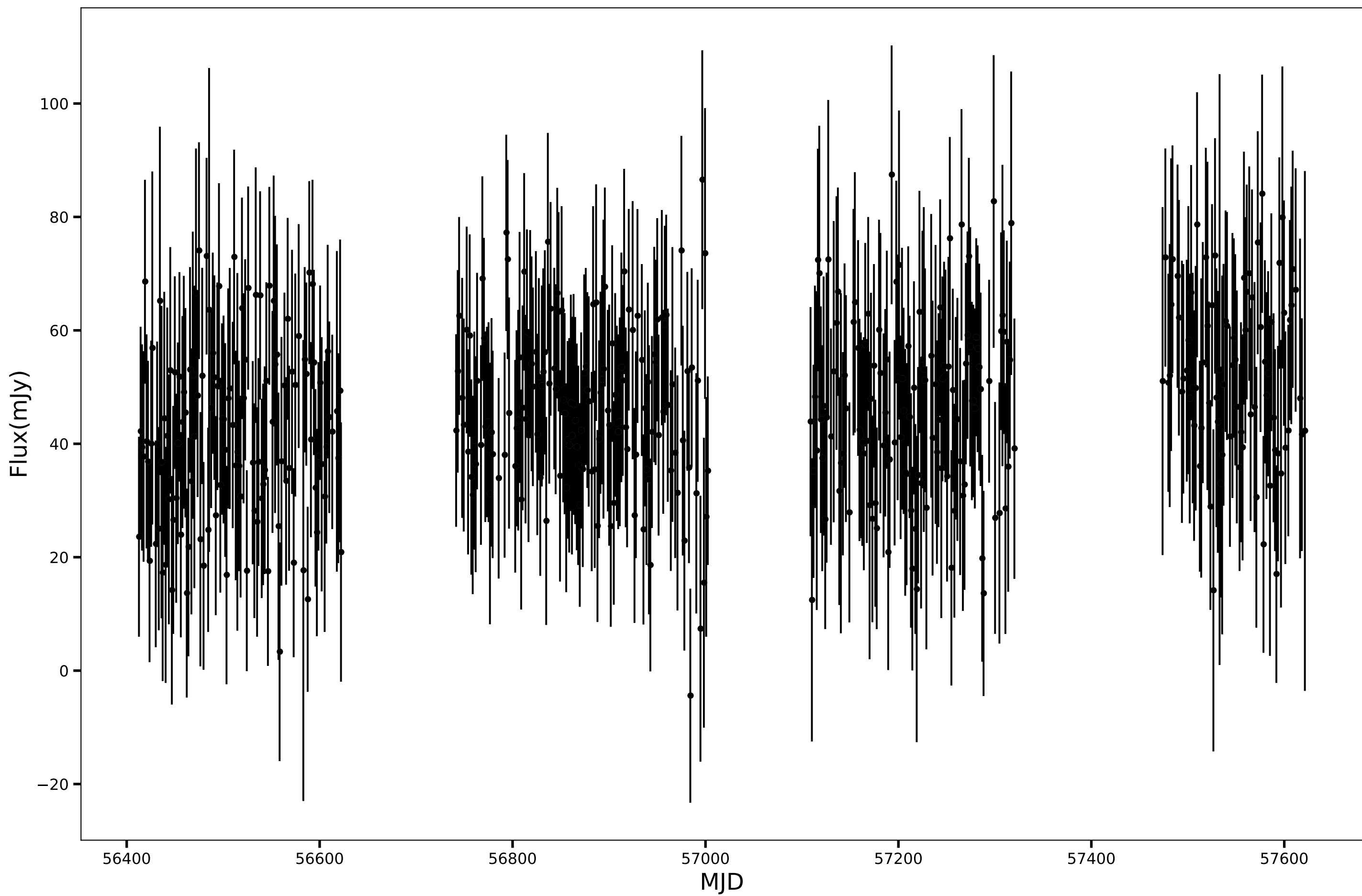
SPT-SJ234442-6108.2, RA=356.1752d, DEC=-61.1380d, mean_flux=46.33 (mJy), 90GHz
