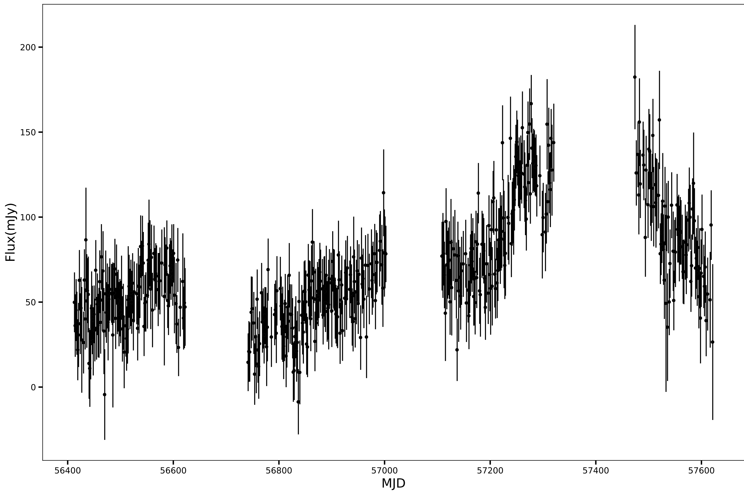
SPT-SJ233726-5901.1, RA=354.3605d, DEC=-59.0184d, mean_flux=68.64 (mJy), 90GHz
