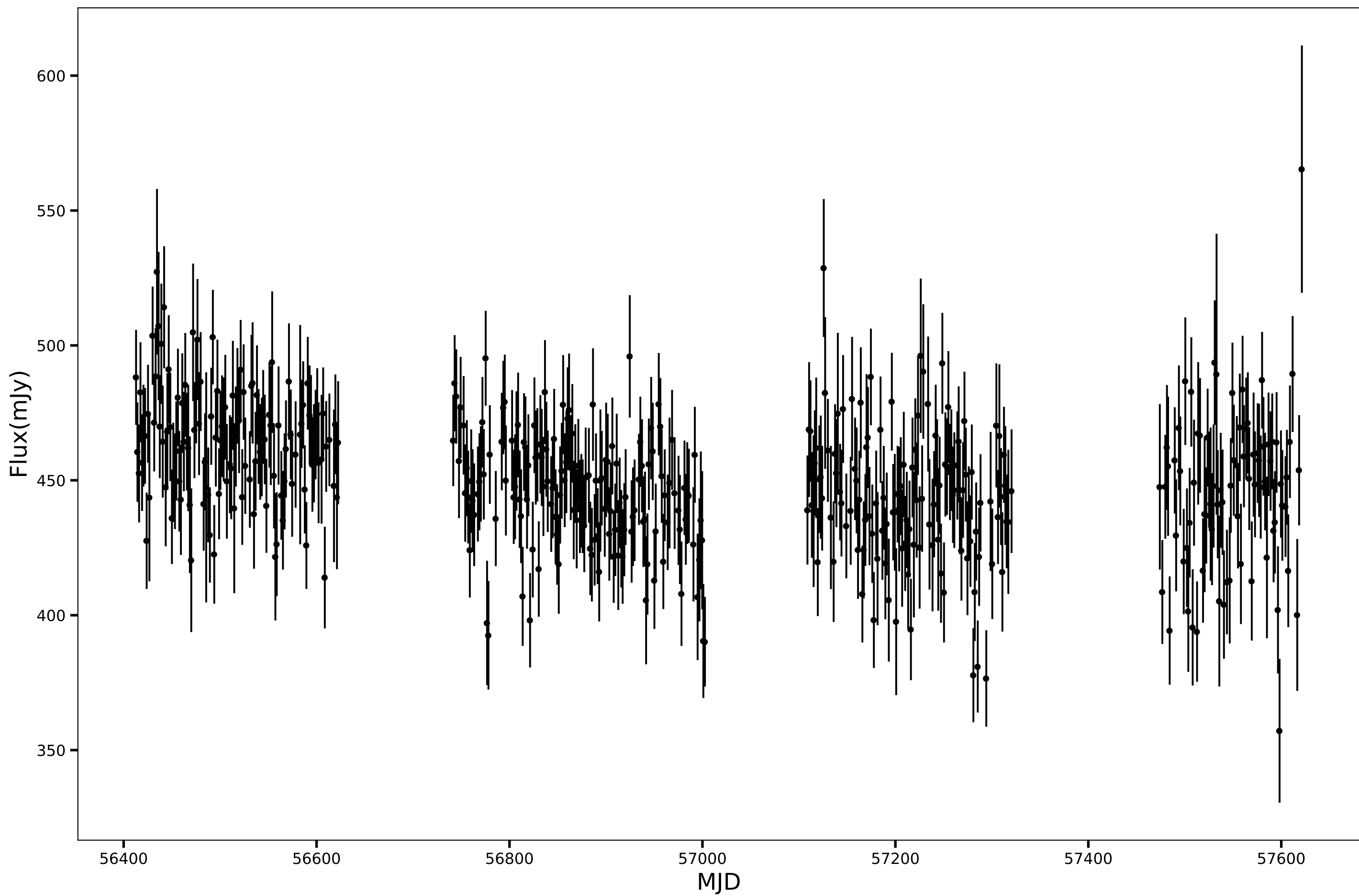
SPT-SJ233612-5236.3, RA=354.0502d, DEC=-52.6053d, mean_flux=450.12 (mJy), 90GHz
