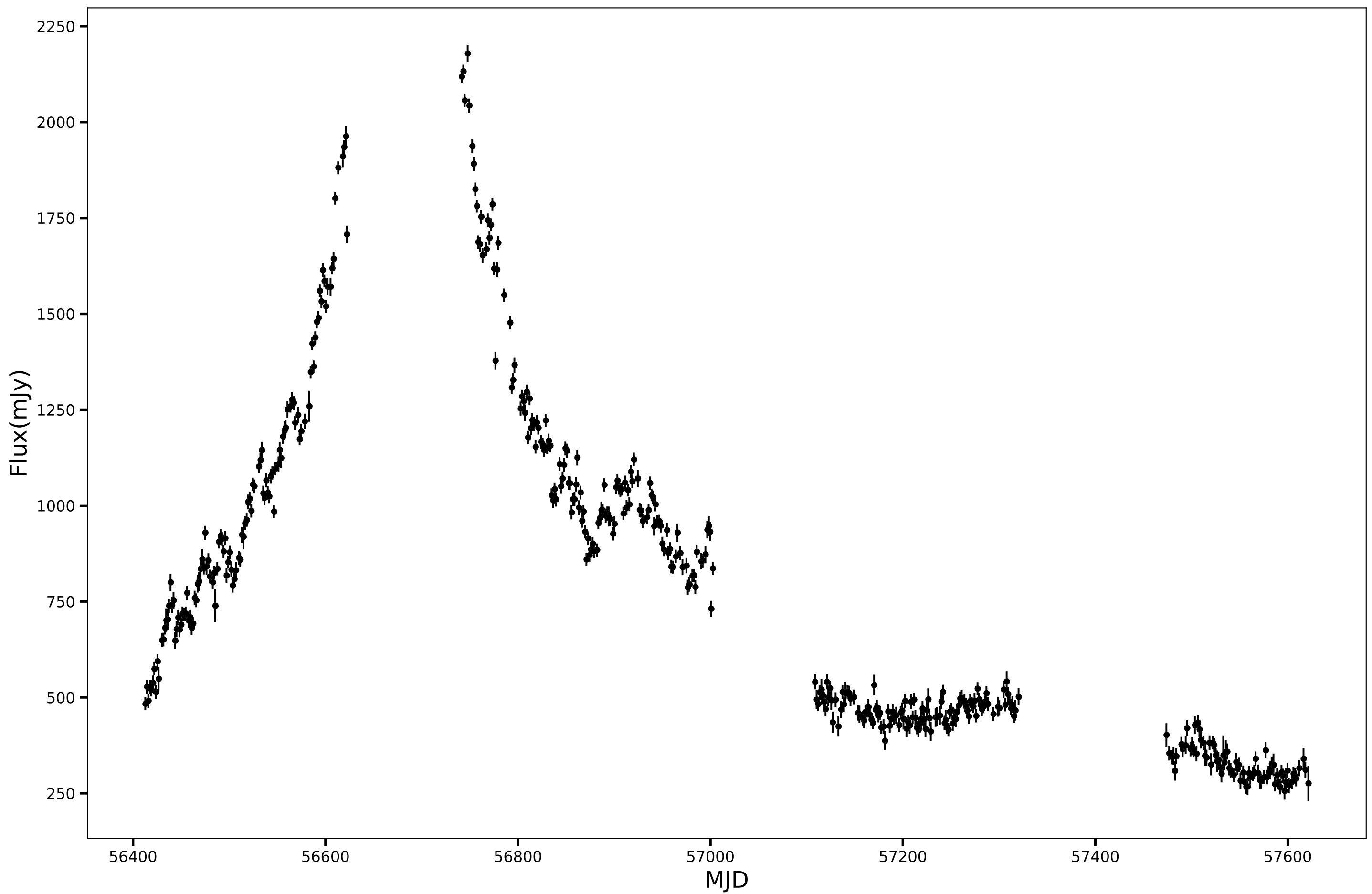
SPT-SJ232920-4955.6, RA=352.3370d, DEC=-49.9276d, mean_flux=795.21 (mJy), 90GHz
