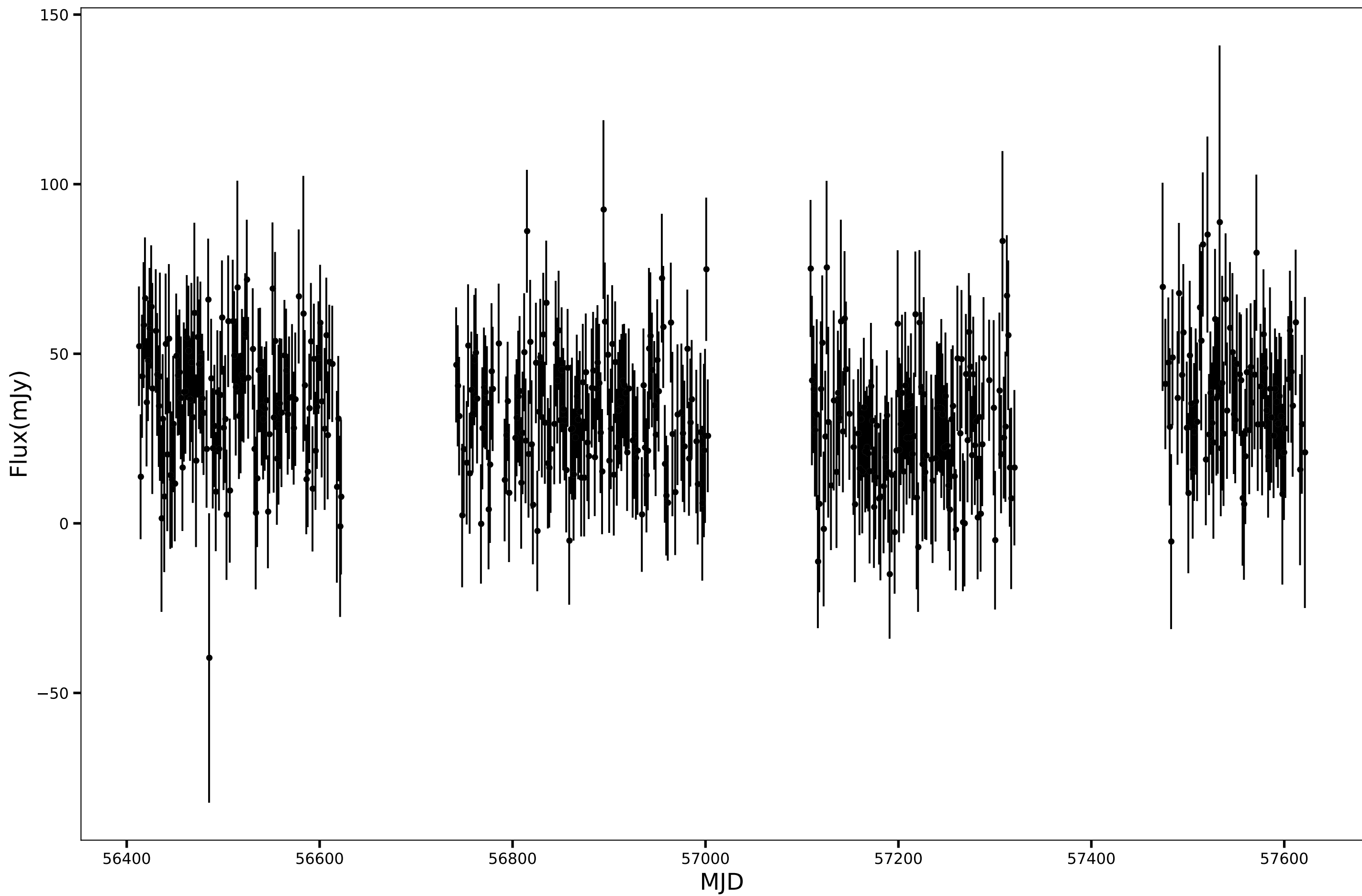
SPT-SJ232804-5630.0, RA=352.0201d, DEC=-56.5005d, mean_flux=33.14 (mJy), 90GHz
