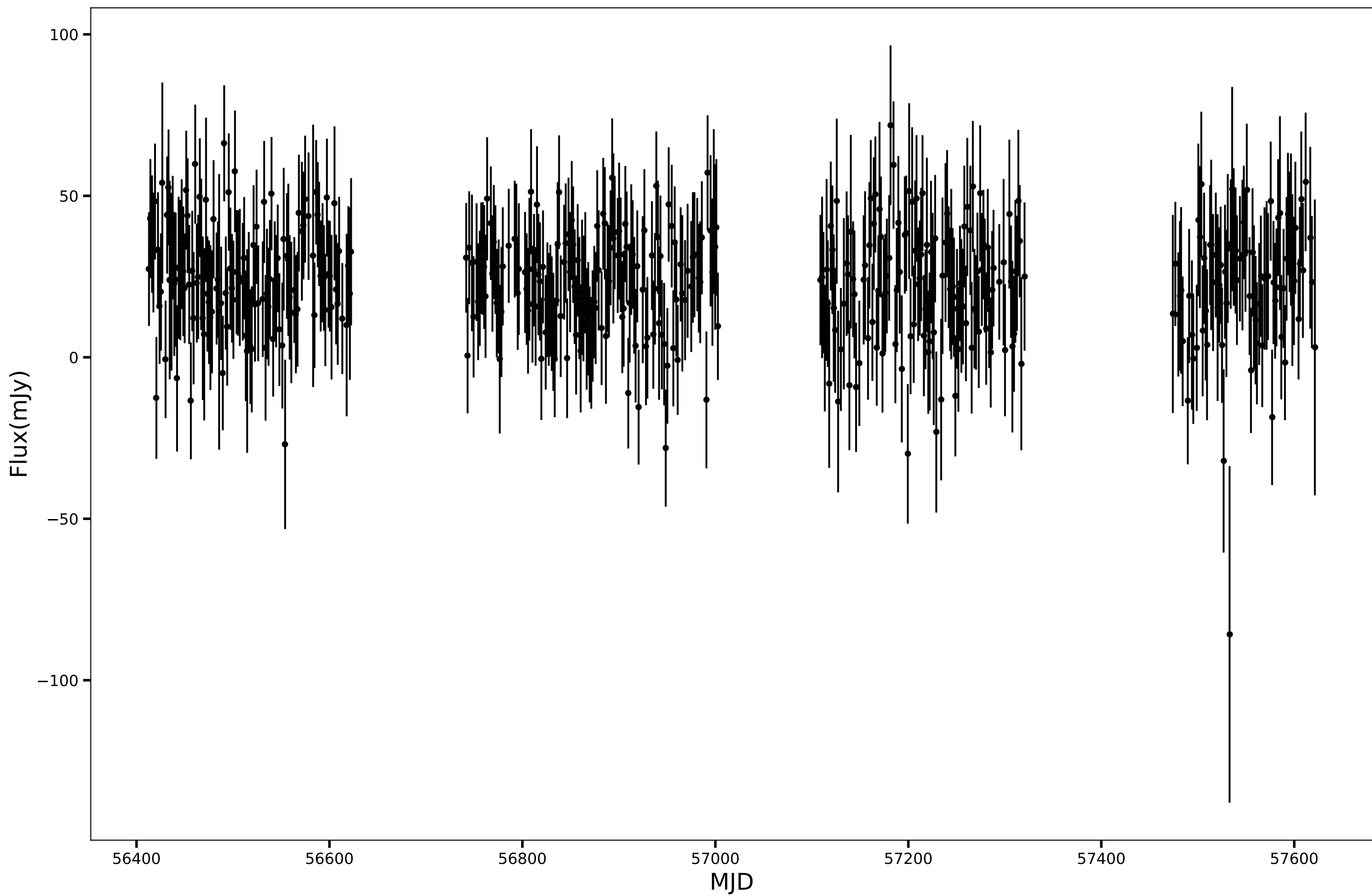
SPT-SJ232510-5656.4, RA=351.2957d, DEC=-56.9409d, mean_flux=23.32 (mJy), 90GHz
