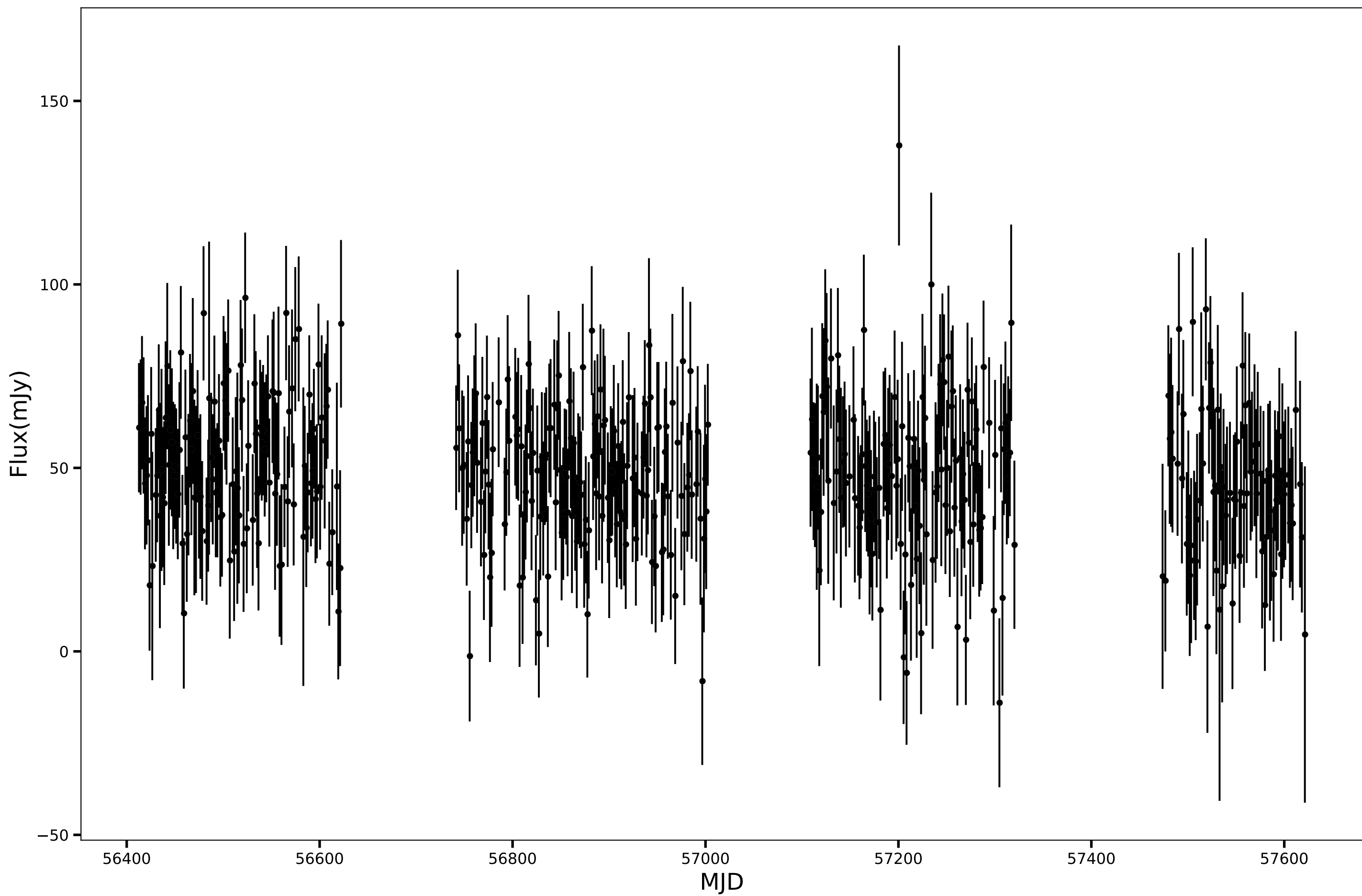
SPT-SJ232252-5322.0, RA=350.7189d, DEC=-53.3667d, mean_flux=48.41 (mJy), 90GHz
