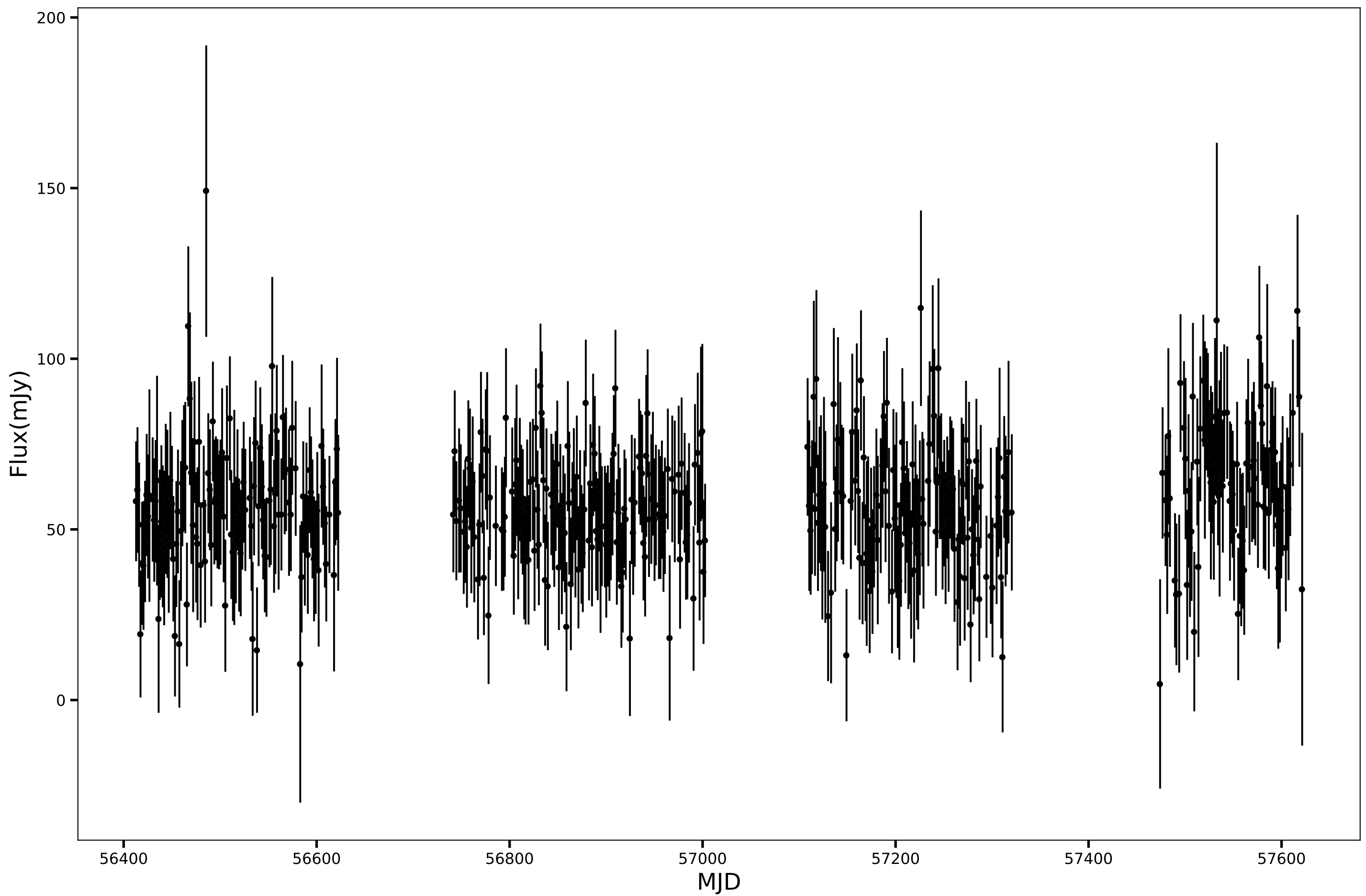
SPT-SJ232142-6438.1, RA=350.4284d, DEC=-64.6362d, mean_flux=57.27 (mJy), 90GHz
