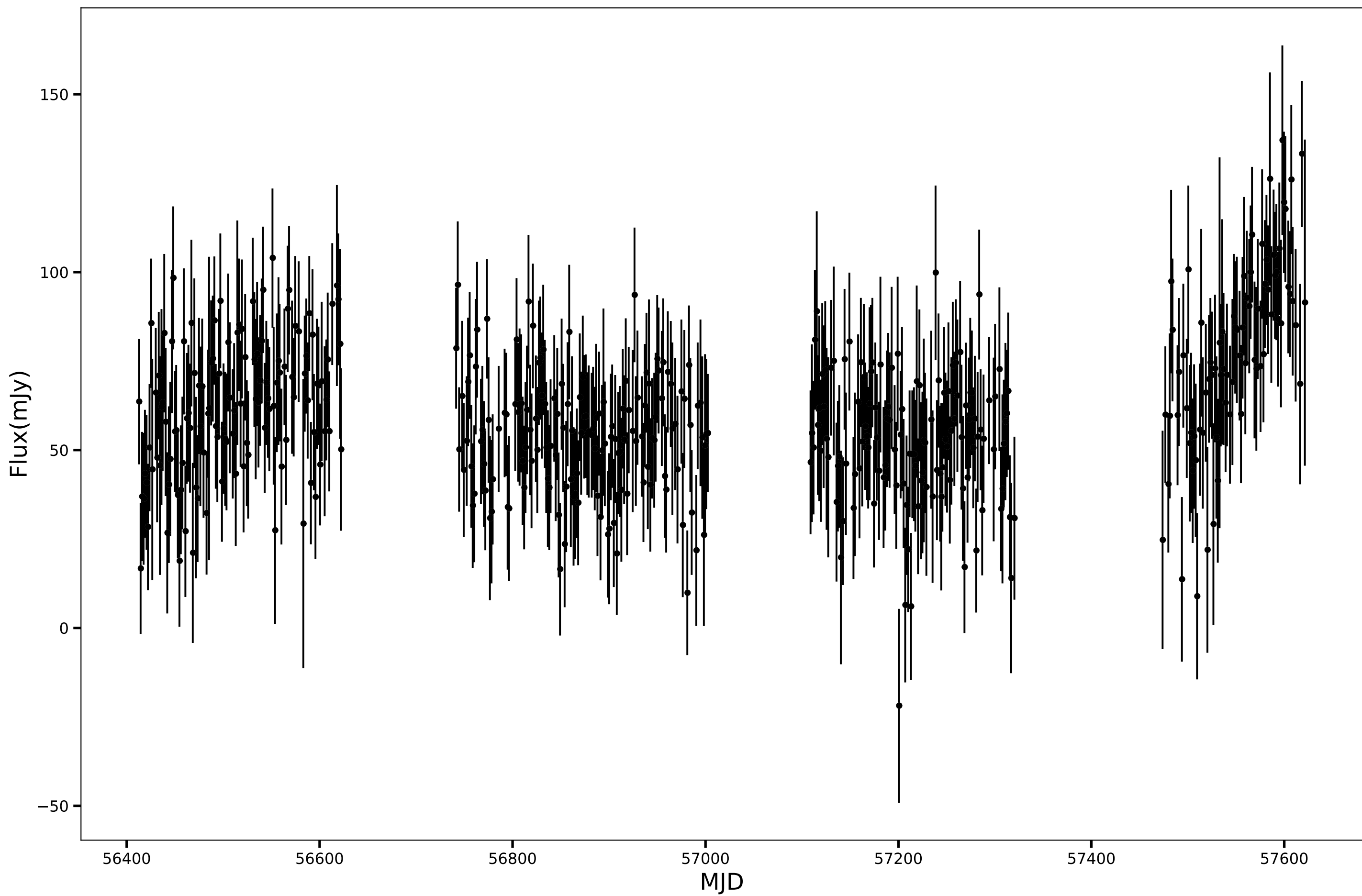
SPT-SJ232100-5402.5, RA=350.2506d, DEC=-54.0424d, mean_flux=59.92 (mJy), 90GHz
