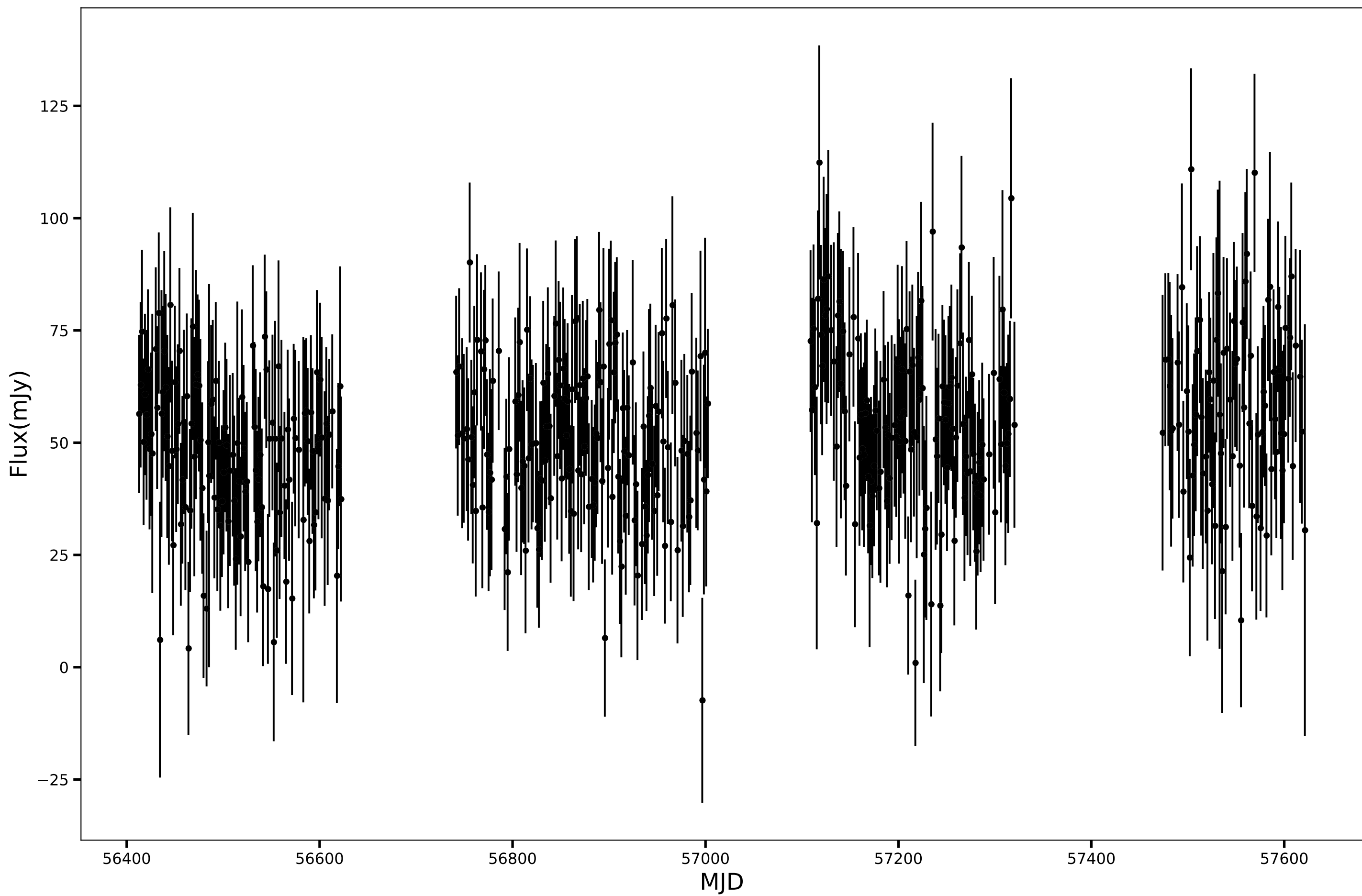
SPT-SJ231916-5331.8, RA=349.8185d, DEC=-53.5308d, mean_flux=52.33 (mJy), 90GHz
