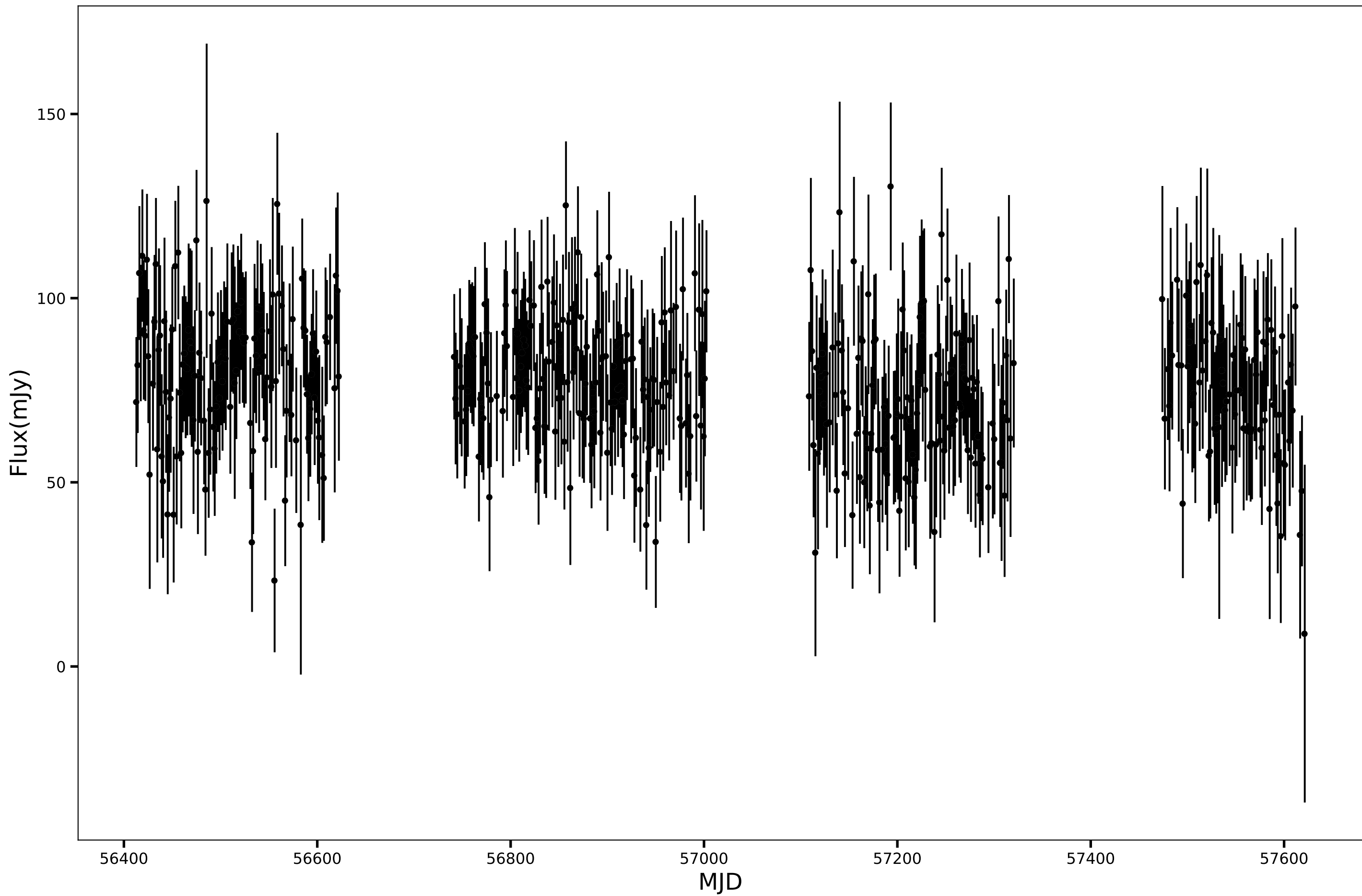
SPT-SJ231716-6215.3, RA=349.3194d, DEC=-62.2563d, mean_flux=76.59 (mJy), 90GHz
