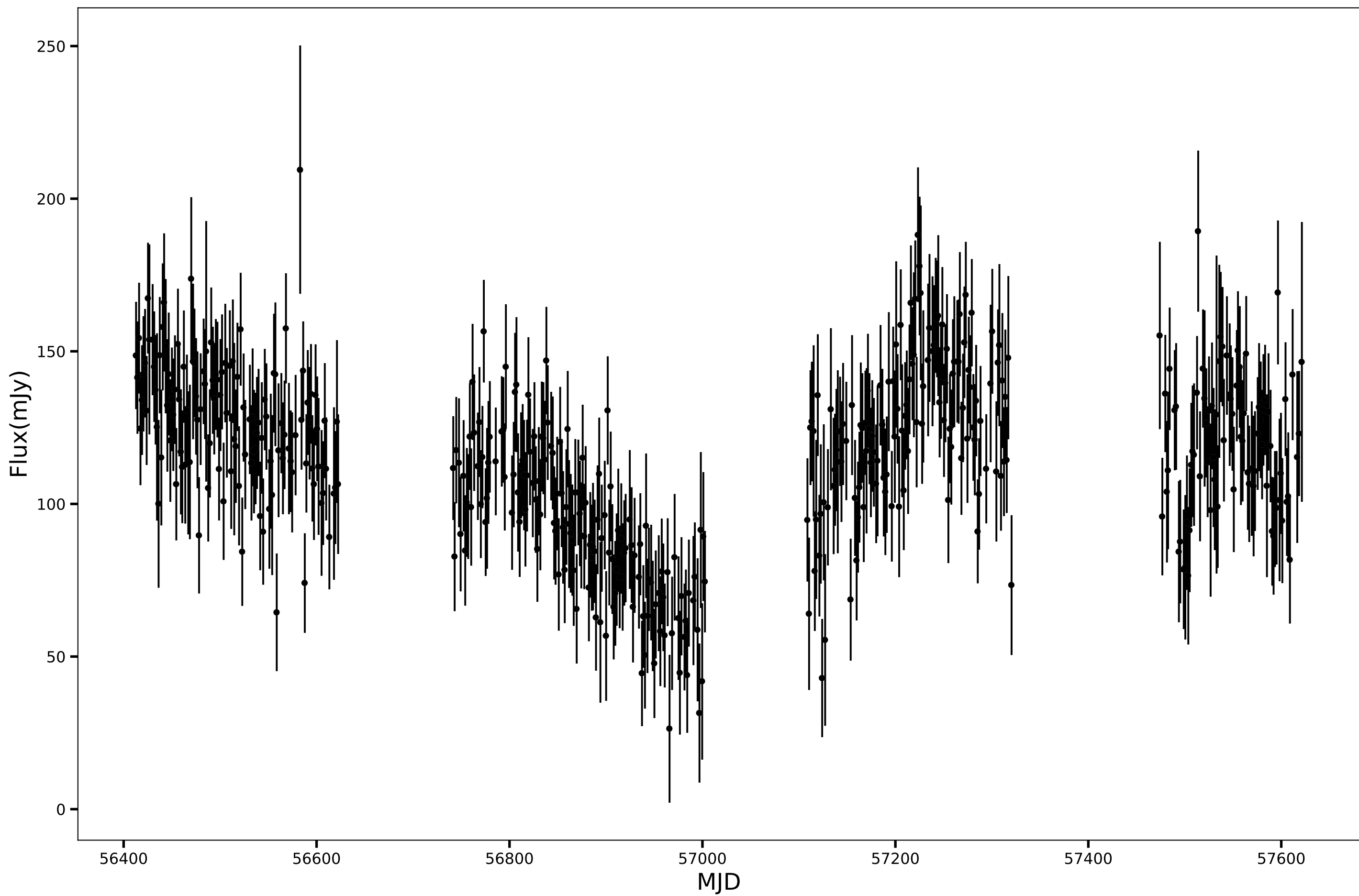
SPT-SJ230903-5050.9, RA=347.2637d, DEC=-50.8494d, mean_flux=114.87 (mJy), 90GHz
