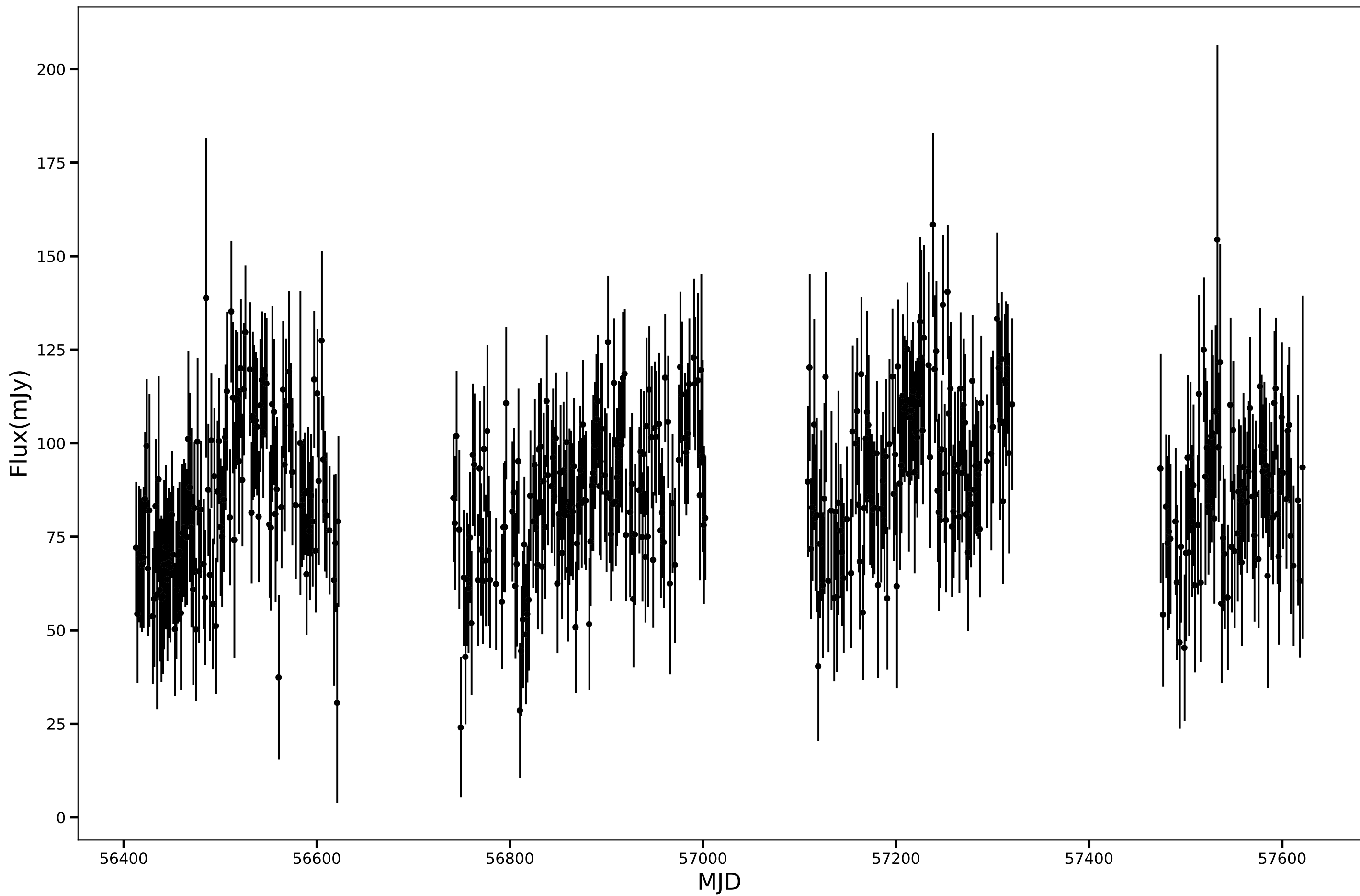
SPT-SJ230137-5913.2, RA=345.4042d, DEC=-59.2211d, mean_flux=87.90 (mJy), 90GHz
