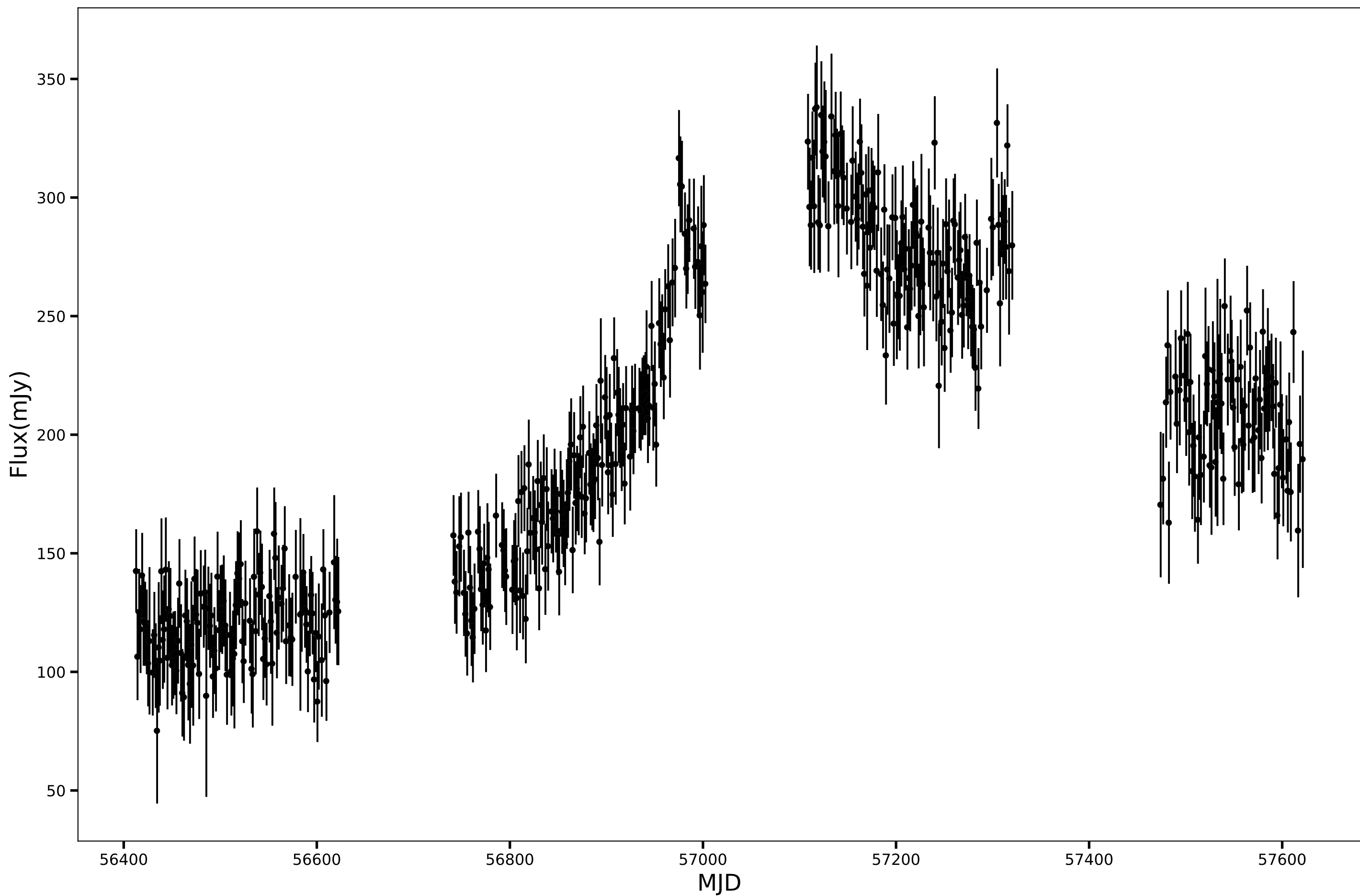
SPT-SJ225457-5925.9, RA=343.7403d, DEC=-59.4318d, mean_flux=197.97 (mJy), 90GHz
