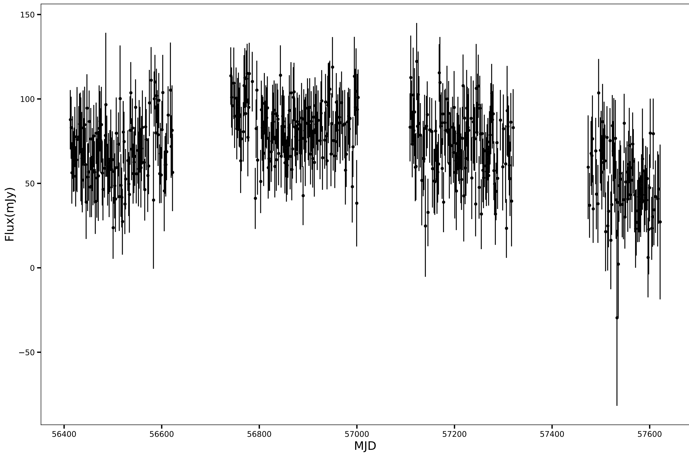
SPT-SJ225423-5148.7, RA=343.5990d, DEC=-51.8118d, mean_flux=71.02 (mJy), 90GHz
