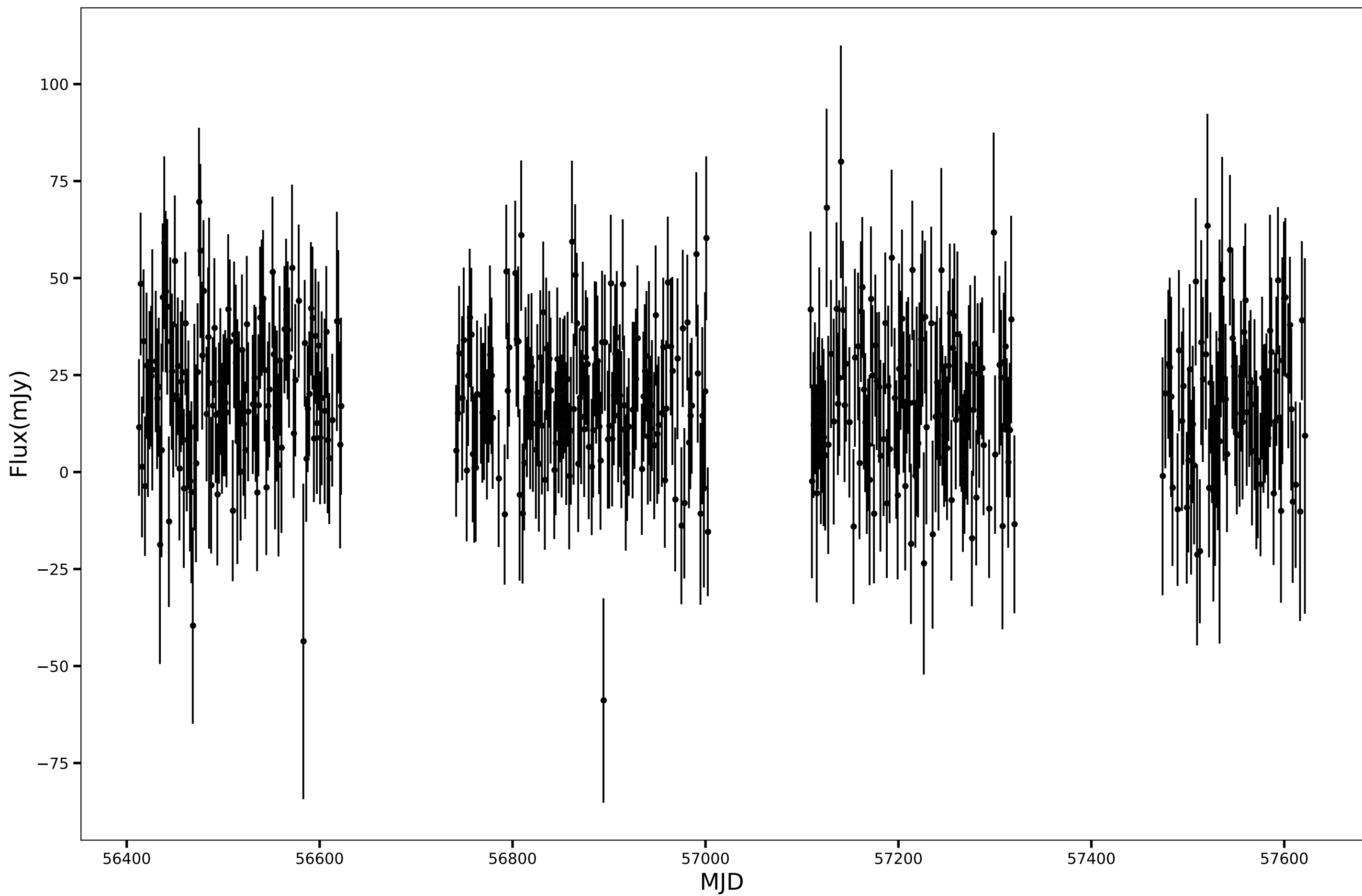
SPT-SJ225400-5025.1, RA=343.5014d, DEC=-50.4193d, mean_flux=18.91 (mJy), 90GHz
