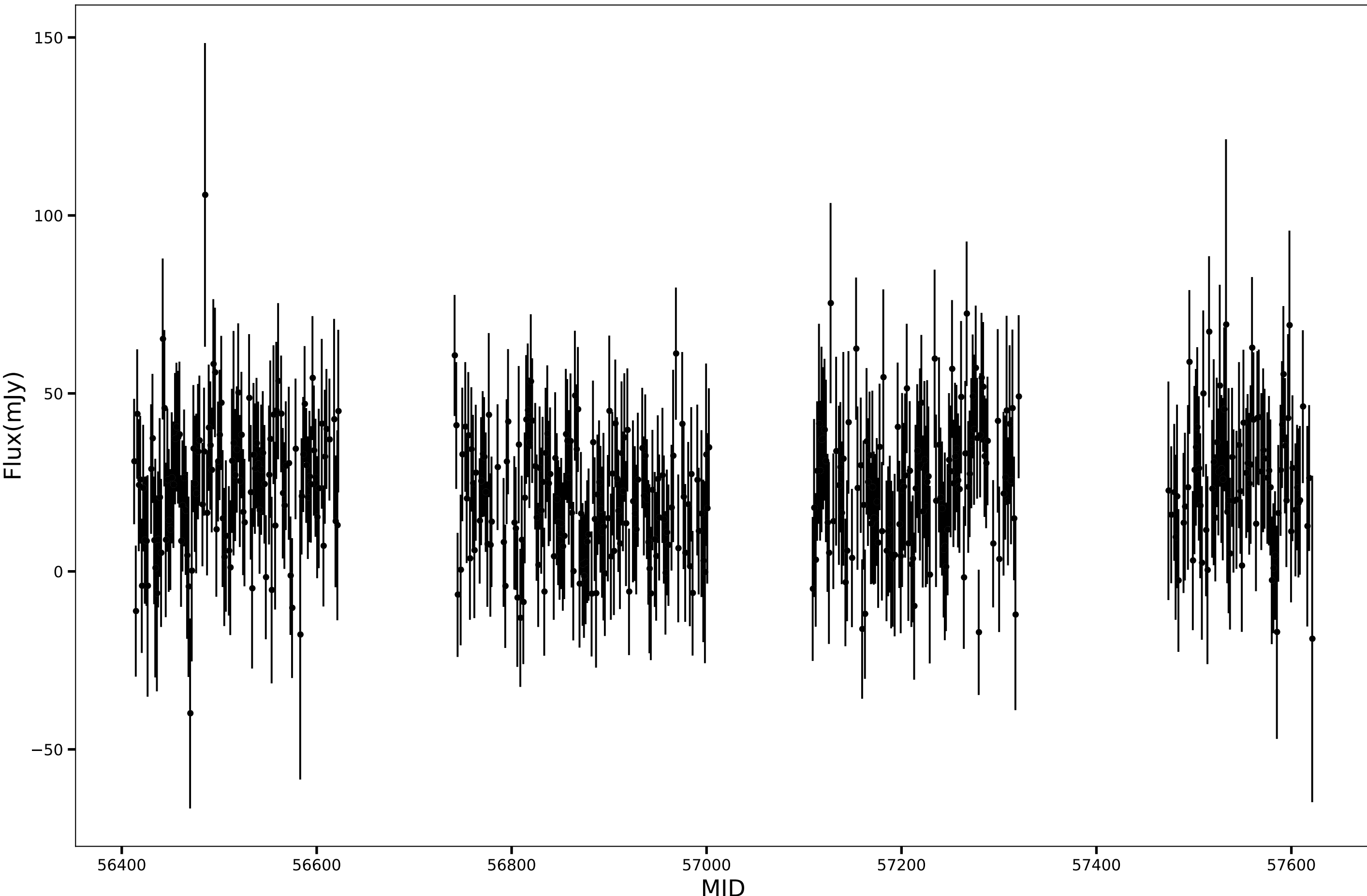
SPT-SJ225139-5801.0, RA=342.9141d, DEC=-58.0170d, mean flux=23.30 (mJy), 90GHz
