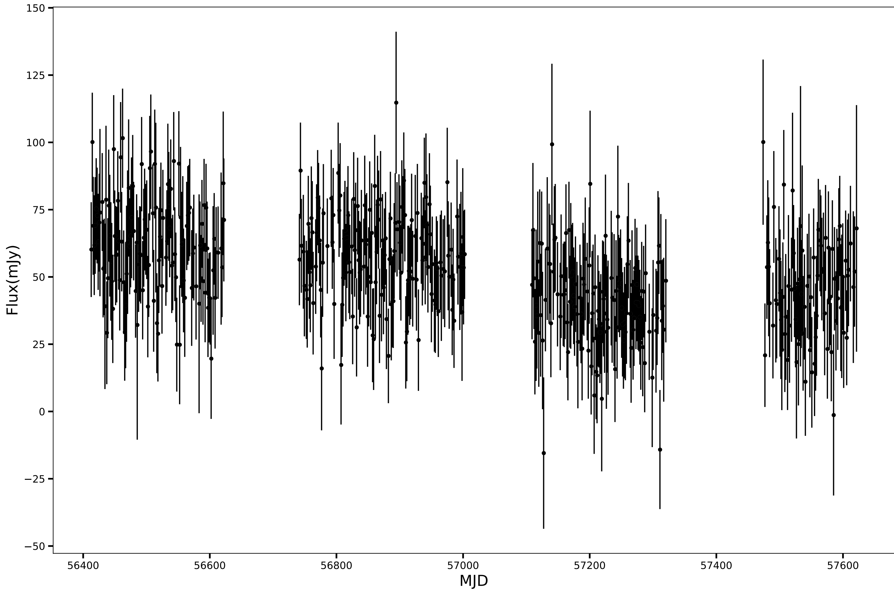
SPT-SJ225136-5453.0, RA=342.9017d, DEC=-54.8844d, mean_flux=52.06 (mJy), 90GHz
