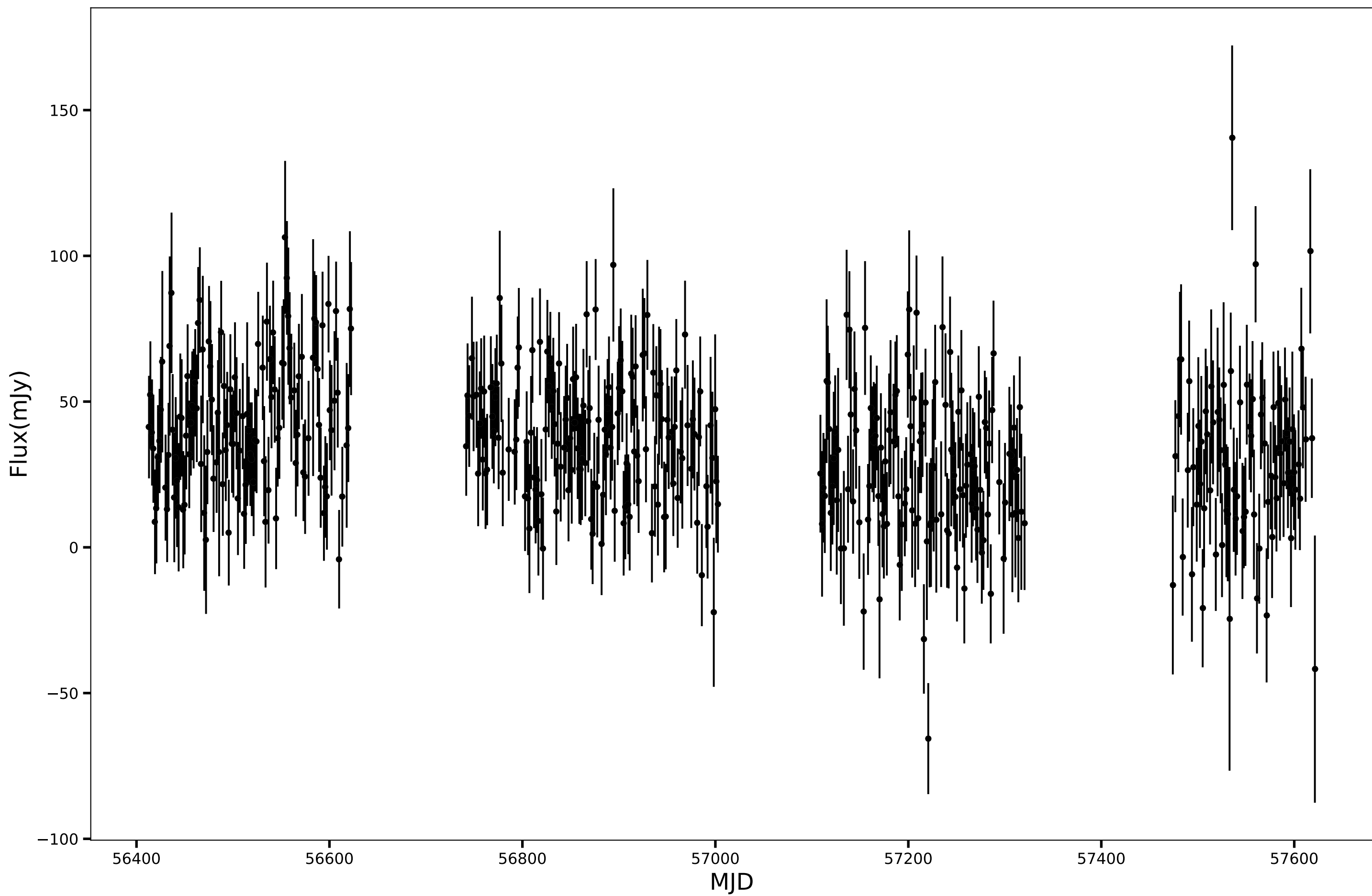
SPT-SJ224500-4931.8, RA=341.2518d, DEC=-49.5302d, mean_flux=35.12 (mJy), 90GHz
